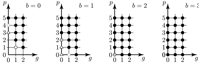
Fig. 1. The behaviour of \Delta_k(\Sigma) when b \leq 3, g \leq 2 and p \leq 5 . Symbols indicate the behaviour of \Delta_k(\Sigma) as k goes to infinity: solid disks indicate exponential behaviour, striped disks polynomial behaviour, solid circles that \Delta_k(\Sigma) = 1 , and dotted circles represent unsolved cases. Triangles mean that \mathcal{F}(\Sigma) is finite. When b = 0 and there is no symbol, \mathcal{F}(\Sigma) is empty.
