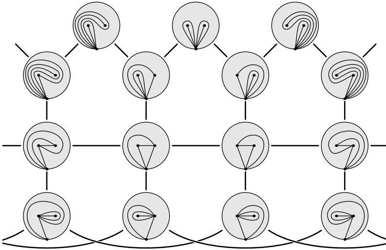
Fig. 7. A portion of the flip-graph of a 2-punctured disk with one marked point in the boundary.
