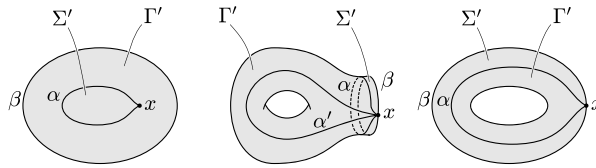
Fig. 4. The constructions in Propositions 9, 10 and 11.
