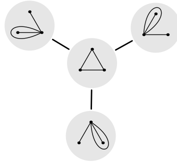
Fig. 2. The flip-graph of a 3-punctured sphere.
