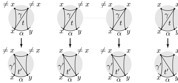
Fig. 6. The flip between T and T' .
