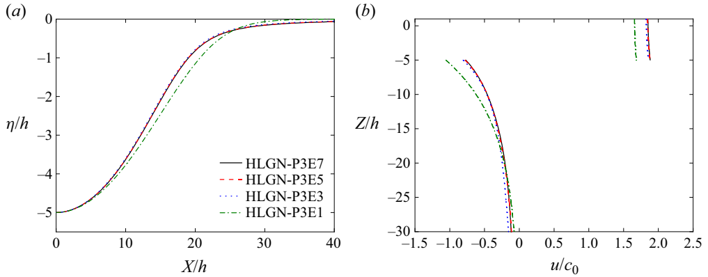
Figure 9. Convergence test of the present HLG models for different levels, \lambda = 2\lambda_{e-MCC} , \rho_2/\rho_1 = 0.78 and a/h = 5 : (a) wave profile; (b) velocity profile at the maximum interface displacement.
