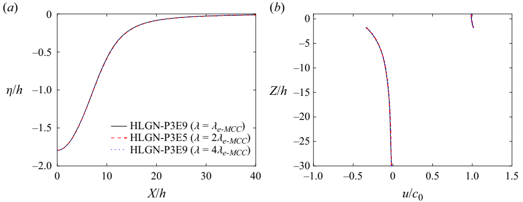
Figure 8. Comparisons between the converged results of the present HLG models with different representative wavelength \lambda , \rho_2/\rho_1 = 0.78 and a/h = 1.7955 : (a) wave profile; (b) velocity profile at the maximum interface displacement.
