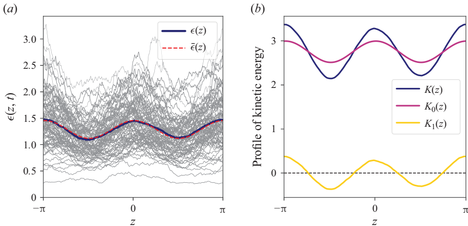
Figure 3. (a) Instantaneous profile of \epsilon(z, t) = \langle \epsilon(\mathbf{x}, t) \rangle_\perp . The time-averaged profile \epsilon(z) = \langle \epsilon(\mathbf{x}, t) \rangle_{\perp, t} is also shown. The red dashed line denotes \bar{\epsilon}(z) , a sinusoidal fitting of \epsilon(z) by (2.31). (b) Time-averaged profile of kinetic energy with fluctuating velocity K(z) , and its equilibrium K_0(z) and non-equilibrium K_1(z) contributions. See the main text and Appendix B for the definition.
