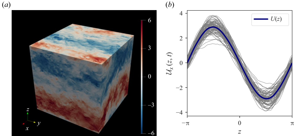
Figure 2. (a) Instantaneous distributions of U_x(\mathbf{x}, t) at Re_\lambda = 184 . Blue (red) corresponds to the negative (positive) value of U_x . (b) Instantaneous profiles of U_x(z, t) = \langle U_x(\mathbf{x}, t) \rangle_\perp in grey. Time-averaged profile U(z) = \langle U_x(\mathbf{x}, t) \rangle_{\perp, t} is indicated by a thick line.
