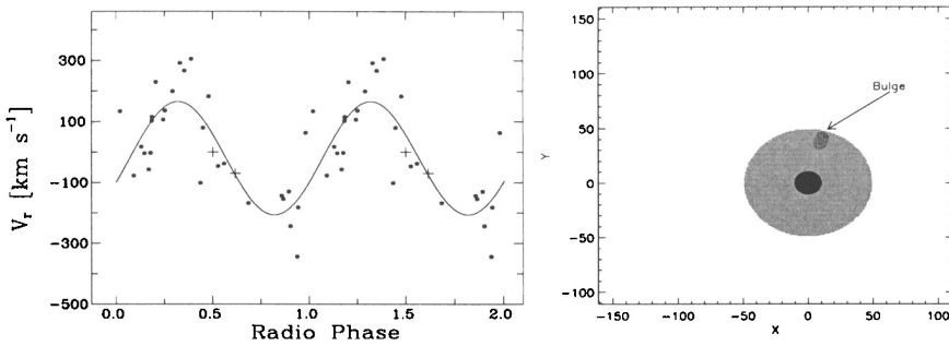
Figure 2. Left panel: Phase plot of the radial velocities of the moving component as a function of radio phase. The solid line is the best cosine fit. The dots represent our data; the crosses are from Paredes et al. (1990). Right panel: Schematic representation of the Be star, its H\alpha -emitting disk, and the bulge located near to the outer edge. The axes are in units of R_{\odot} .
