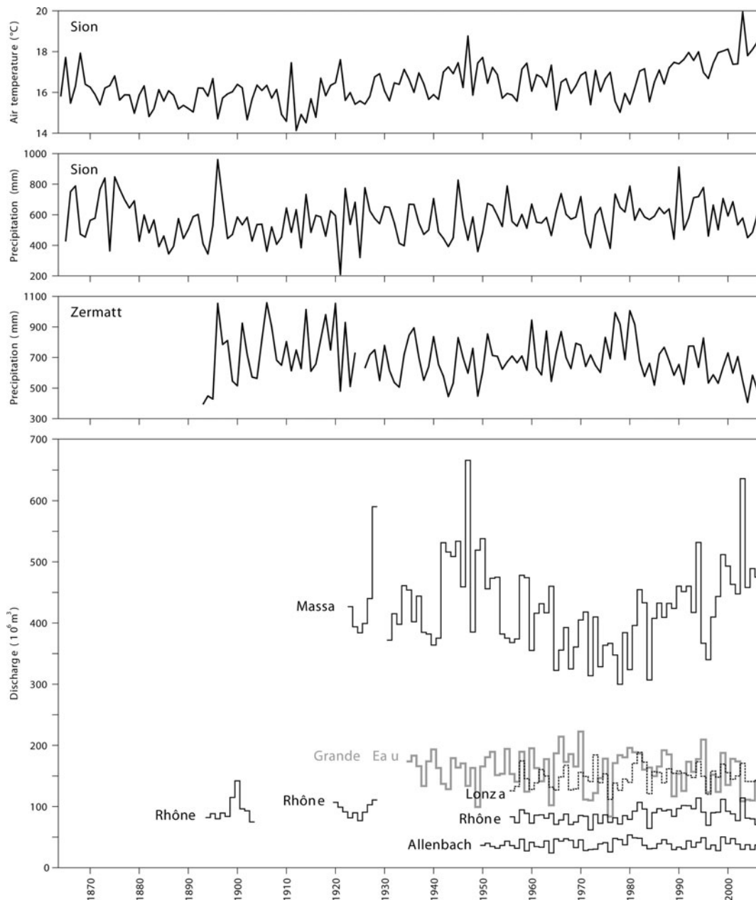
Fig. 3. Year-to-year variations of mean summer air temperature ( T_{5-9} ) at Sion, annual total precipitation between November and October ( P_{11-10} ) at Sion and Zermatt, and annual total discharge between January and December ( Q_{1-12} ) of the Allenbach, Grande Eau, Lanza, Massa and Rhône in the period 1866–2006. Discharge measurements of the Massa were interrupted in 1929 and 1930, and two short discrete periods of measurement preceded the continuous record of the Rhône.
