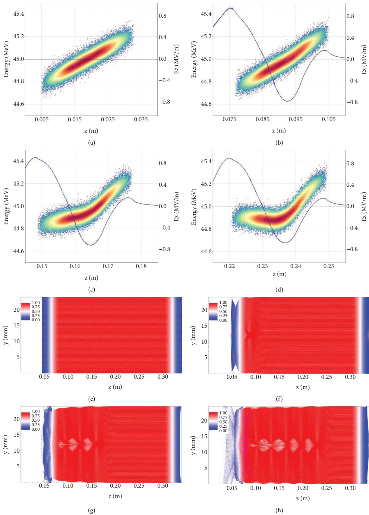
FIGURE 4: (a–d) Beam longitudinal phase space (dot) and longitudinal plasma wakefield E_z (blue line). (e–h) The corresponding electron distribution in plasma. (a) Initial bunch energy distribution. (e) Initial electron distribution in plasma. (b, f) Propagation distance of bunch s = 7.2 cm. (c, g) Propagation distance of bunch s = 14.4 cm. (d, h) Propagation distance of bunch s = 21.6 cm.
