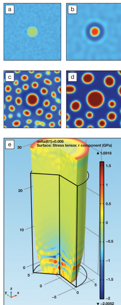
(a-d) A series of images from a simulation of spinodal decomposition, nucleation, growth, and coarsening was incorporated into a class on kinetics and phase transformations in materials science and engineering using the COMSOL software. (e) An image from a COMSOL simulation of plastic necking was incorporated into a class on the mechanical properties of materials. Images courtesy of Michael Falk, Johns Hopkins University.
