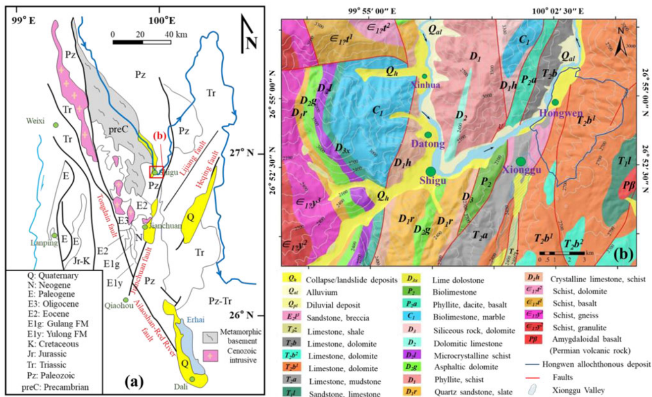
Figure 2. (a) Simplified geological map of southeastern Tibetan Plateau showing main faults, distributions of strata and intrusions, and the course of the Jinsha River (revised from Wei et al., 2016); location of Figure 2b shown with red box. (b) Geological map of the First Bend of the Yangtze River (FBYR).
