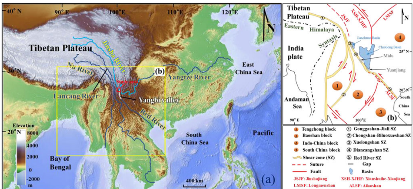
Figure 1. (a) Digital elevation model map showing major rivers of Southeast Asia. (b) Tectonic framework of southeastern Tibetan Plateau.
