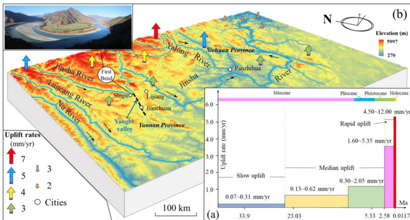
Figure 3. (a) Uplift rates of the Qinghai Tibet Plateau, revised from Zhan et al. (2018). (b) Vertical uplift velocity in northwest Yunnan with respect to the Sichuan basin (referenced from Hao et al., 2014); inset shows photographic image of the FBYR.
