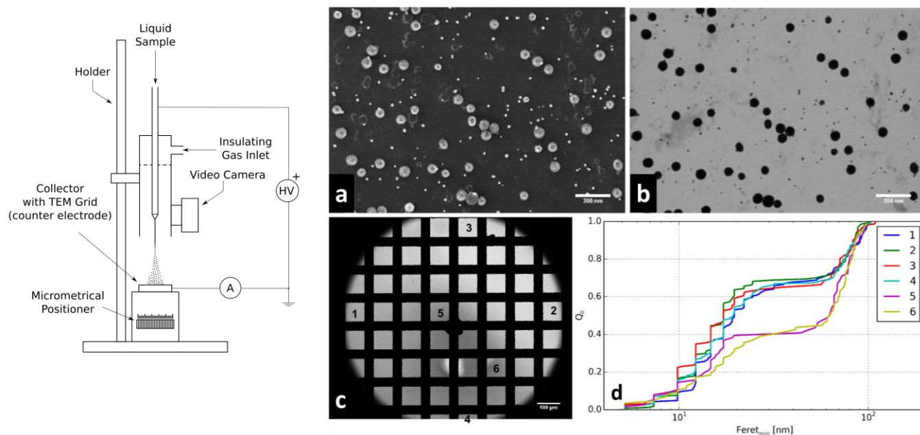
Figure 1. left: The principle of electrospray deposition system; right: a) SEM micrograph of a bimodal silica suspension (certified reference material ERM FD102 with particle sizes 18.2 nm and 84.0 nm), b) same area as (a) in STEM mode (at SEM); c) images of ERM FD102 on TEM grid were recorded on different locations, and d) the respective particles size distributions have been evaluated.
