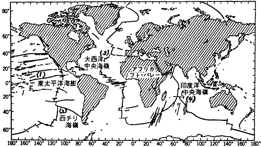
Fig. 2. Ocean Ridges and Fracture Zones
