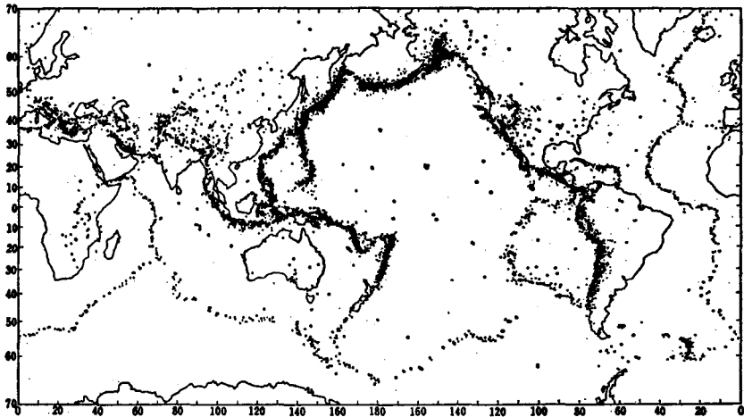
Fig. 3 Earthquakes occurring at shallow hypocentres during 1961-67 (After M. Barazangi and J. Dorman)
