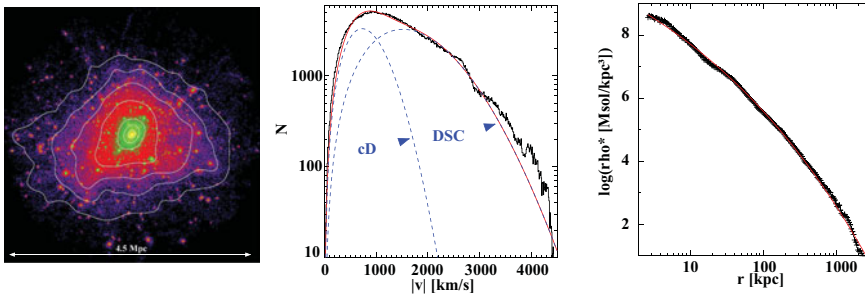
Figure 1. Stellar density map of the most massive cluster (color coded). The white contours show the diffuse stellar component plus the central galaxy (cD) after subtracting the stars from the other cluster member galaxies. Middle: Distribution of the stellar velocities for the DSC and the cD galaxy (black histogram) with a double Maxwellian fit (red line). Right: Radial stellar density profile of DSC and cD (black symbols) with a single Sérsic profile fit (red line).
