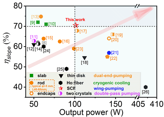
Figure 1. Overview of 2- \mu m continuous-wave (CW) Ho:YAG and Ho: fiber lasers [8–26] .
