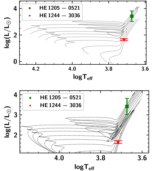
Figure 3. The locations of HE 1205–0521, and HE 1244–3036 in the H-R diagram are shown. The evolutionary tracks for 0.7, 0.9, 1.2, 1.6, 1.9, 2.2, 2.5, 3, and 3.5 M_{\odot} are shown from bottom to top in the upper panel. The isochrone tracks for \log(\text{age}) 10.25, 10.05, 9.85, 9.45, 9.15, 8.95, 8.8, 8.65, 8.54 and 8.45 are shown from bottom to top in the bottom panel.
