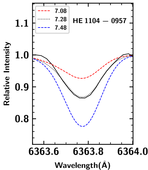
Figure 4. Synthesis of [OI] line around 6363 Å in HE 1104–0957. The dotted line represents synthesized spectra, and the solid line indicates the observed spectra. Red short dashed line represents the synthetic spectra corresponding to \Delta[O/Fe] = -0.2 and blue short dashed line corresponds to \Delta[O/Fe] = +0.2
