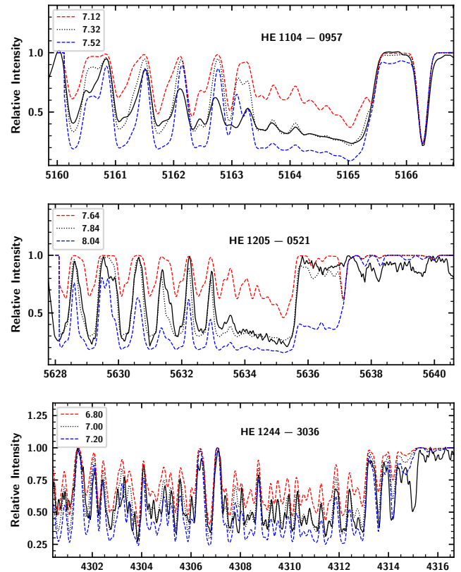
Figure 5. Synthesis of C_2 band around 5165, 5635 Å, and CH band around 4315 Å. The dotted line represents synthesized spectra, and the solid line indicates the observed spectra. Red short dashed line represents the synthetic spectra corresponding to \Delta[C/Fe] = -0.2 and blue short dashed line corresponds to \Delta[C/Fe] = +0.2
