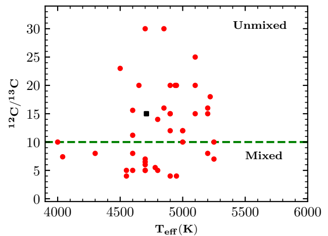
Figure 13. The location of HE 1205–0521 (filled square) in the ^{12}C/^{13}C vs. T_{eff} diagram. The filled circles represent the stars from Spite et al. 2006 and Aoki et al. 2007
