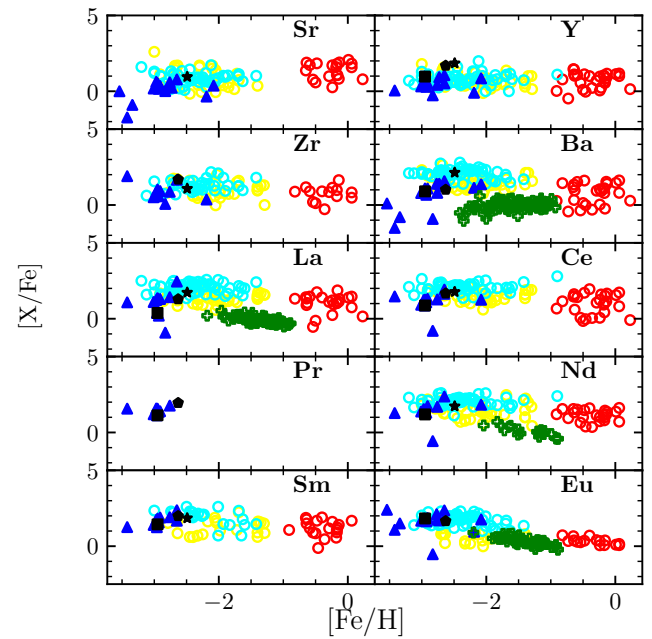
Figure 9. Same as Figure 8, but for heavy elements.
