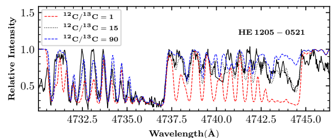
Figure 6. Spectral synthesis fits of the C_2 features around 4740 Å in HE 1205–0521. The solid line indicates the observed spectra. Short and long dashed lines are shown to illustrate the sensitivity of the line strengths to the isotopic carbon abundance ratios
