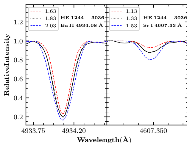
Figure 7. Synthesis of Ba II around 4934.08 Å, and Sr II around 4607.33 Å in HE 1244–3036. The dotted line represents synthesized spectra, and the solid line indicates the observed spectra. Red short dashed line represents the synthetic spectra corresponding to \Delta[\text{X}/\text{Fe}] = -0.2 and blue short dashed line corresponds to \Delta[\text{X}/\text{Fe}] = +0.2 .
