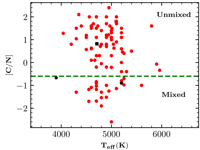
Figure 12. Positions of the programme stars in the [C/N] vs. T_{eff} diagram. Symbols used for the programme stars are the same as in previous Figures. Filled circles represent the stars from prior works (Spite et al. 2006; Aoki et al. 2007; Goswami, Aoki, and Karinkuzhi 2016; T. T. Hansen et al. 2016a; C. J. Hansen et al. 2019; Purandardas et al. 2019; Purandardas, Goswami, and Doddamani 2019; Goswami, Rathour, and Goswami 2021a; Shejeelammal, Goswami, and Shi 2021)
