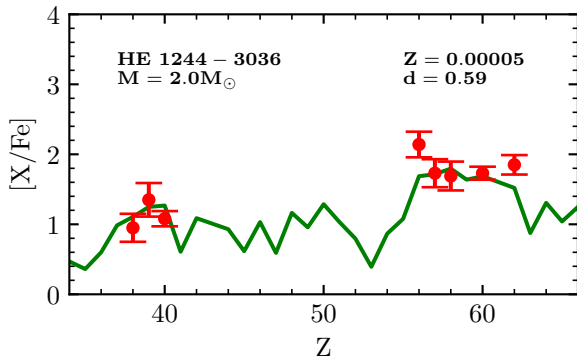
Figure 11. Best-fitting FRUITY model (solid green curve) for HE 1244–3036. The points with error bars indicate the observed abundances.
