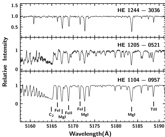
Figure 1. Sample spectra of the three programme stars in the wavelength region 5158–5191 Å are shown. Some features identified are marked on the spectra.
