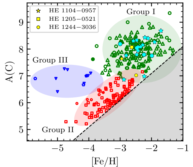
Figure 10. Corrected A(\text{C}) vs. [\text{Fe}/\text{H}] diagram for the compilation of CEMP stars taken from Yoon et al. 2016. Cyan symbols indicate CEMP-r/s stars: binary stars are represented by circles, and stars with no information about the binary status are indicated by "star" symbols. CEMP-s stars are represented using green symbols: open and filled circles indicate binary and single stars, respectively. Stars with no information about the binarity are represented using open triangles. Red symbols represent Group II CEMP-no stars: open and filled hexagons represent binary and single stars, respectively. Stars with no information about the binarity are presented using open squares. Group III CEMP-no stars are represented using red symbols: binary and single stars are represented by open and filled pentagons, respectively. Inverted triangles represent stars with no information about the binary status. The short dashed line represents [\text{C}/\text{Fe}]=0.7 .
