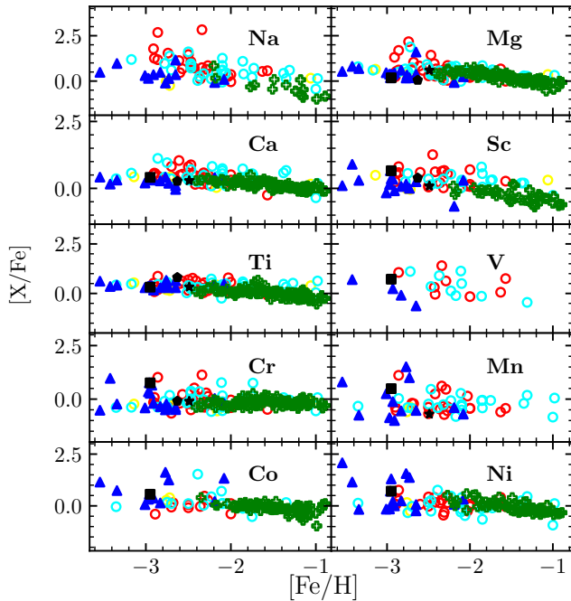
Figure 8. A comparison of the light elements abundance ratios with their counterparts observed in Galactic stars, Sculptor dwarf galaxy stars and Reticulum galaxy stars. Comparisons are shown for elements for which data from prior works are available. Sculptor dwarf galaxy stars from Skúladóttir et al. 2017; Hill et al. 2019. The abundance values for CEMP-no stars used for the comparison are taken from Christlieb et al. 2004, Plez and Cohen 2005, Yong et al. 2013, T. Hansen et al. 2014, Bonifacio et al. 2015, Bessell et al. 2015 and Frebel 2018b. The abundance values for CEMP-s and CEMP-r/s stars are taken from Lucatello et al. 2003, Barklem et al. 2005, Cohen et al. 2006, Goswami et al. 2006, Aoki et al. 2007, Karinkuzhi and Goswami 2015, Purandardas et al. 2019, Purandardas, Goswami, and Doddamani 2019, Shejeelammal, Goswami, and Shi 2021, Purandardas and Goswami 2021 and Goswami, Rathour, and Goswami 2021a. The symbols used are as follows: red circle = CEMP-rs, cyan circles= CEMP-s, yellow circles= CEMP-no, blue triangles = reticulum, black square = HE 1104-0957, black pentagon= HE 1205-0521, black star=HE1244-3036, green plus= sculptor dwarf galaxy
