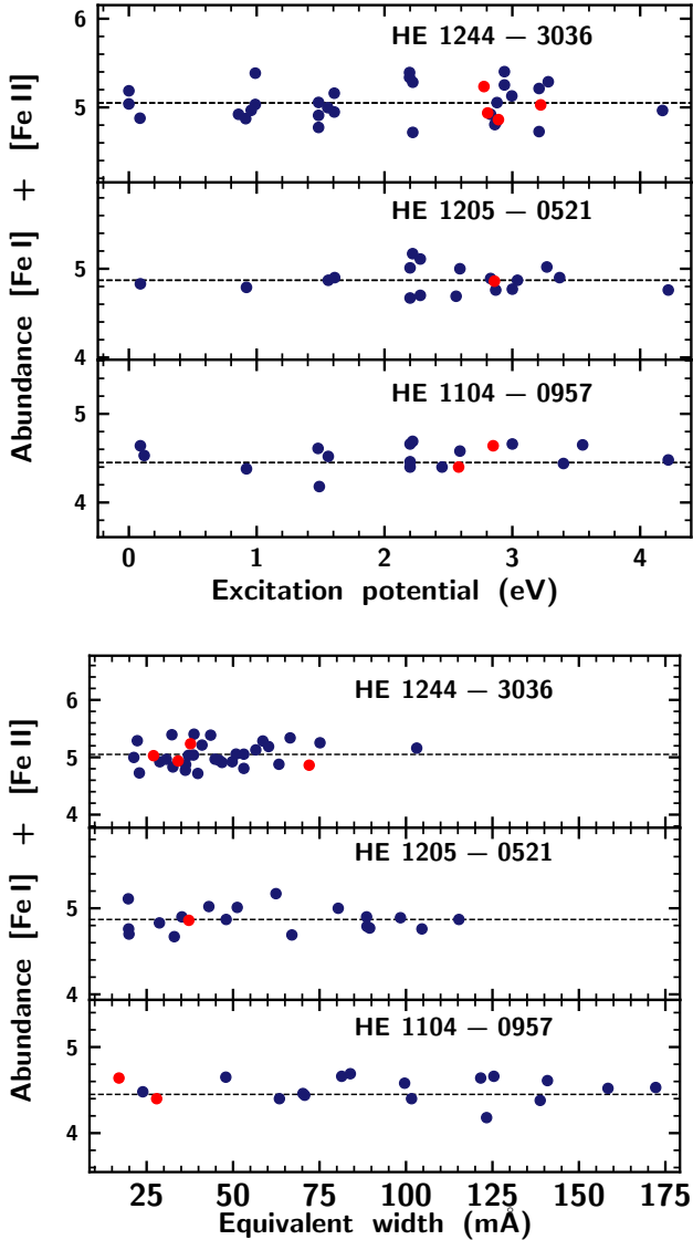
Figure 2. The iron abundances of programme stars as a function of excitation potential (top panel) and equivalent width (bottom panel). In all the panels, the blue-filled circles indicate Fe I lines and the red filled circles represent Fe II lines.
