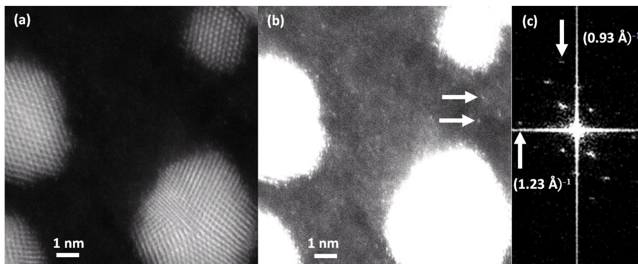
Figure 1. (a) 60 kV monochromated HAADF STEM image of Au nanoparticles on a carbon support, (b) same image, but with the contrast adjusted to show individual Au atoms, two of which are labeled with arrows. (c) FT of a particle in a similar image.
