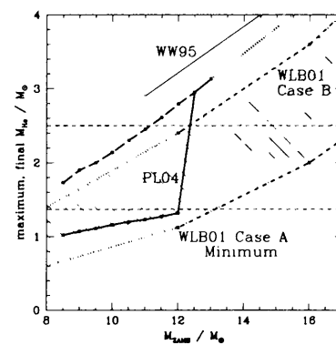
Fig. 2. Final mass (thick solid line) and maximum mass (thick dashed line) of the helium core in single stars as a function of initial mass according to Poelarends & Langer (2004, PL04), extrapolated for initial masses above 12.5 M_{\odot} (the final helium core masses from the calculations of Woosley & Weaver [1995] are indicated by a thin solid line). The hatched region shows the final helium core masses expected in close binaries (from the calculations of Wellstein et al. 2001 [WLB01]). The light dashed horizontal lines give the range for the final helium core mass for which the star may experience an electron-capture supernova. Note that the parameter range for which this may occur for a single star is very small.
