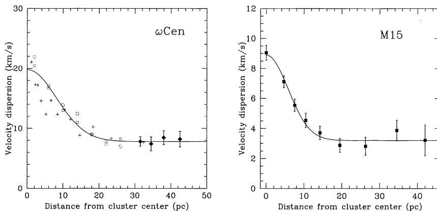
Fig 1. Left: The velocity dispersion profile of \omega Centauri. Proper motion (circles and squares, van Leeuwen et al. 2000) and radial velocities (crosses, Meylan et al. 1995 and Meylan & Mayor 1986) data show the velocity ellipsoid is isotropic. Our radial velocity measurements (diamonds) extend the profile to 45 pc showing the velocity dispersion remains constant for R > 27 \pm 3 pc. Right: Dispersion profile of the globular cluster M15, from data by Drukier et al. (1998). Also in this case the velocity dispersion remains basically constant for R > 18 \pm 3 pc. In both panels the solid line is not a fit to the data. It is meant to illustrate that the velocity dispersion remains constant at large radii.
