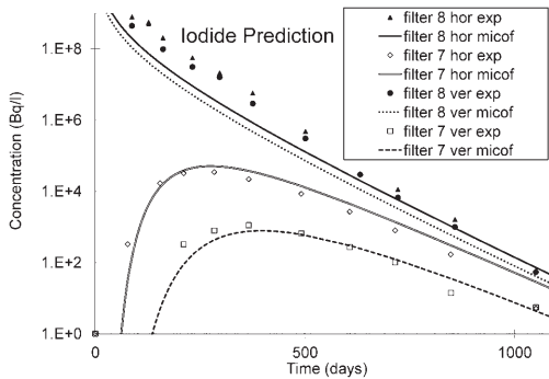
FIG. 14. Blind prediction of the iodide concentration in the TD41HV experiment (hor is the horizontal piezometer, ver is the vertical piezometer).
