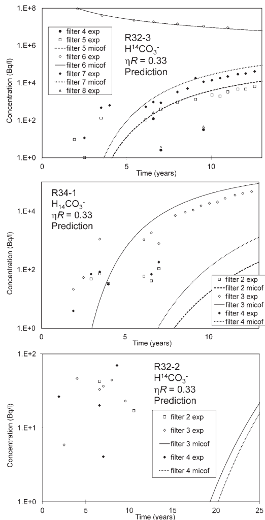
FIG. 12. Blind prediction and experimental data in the filters of the injection piezometer R32-3, the piezometer R34-1 parallel to the injection piezometer, and the inclined piezometer R32-2 of the Tribicarb-3D experiment (tracer: \text{H}^{14}\text{CO}_3^- ). In the filters for which no MICOFF prediction is shown, the prediction is lower than the lowest value in the figure.
