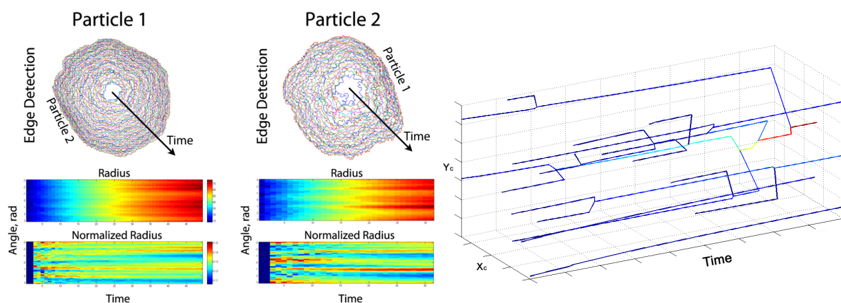
Figure 2. Quantitative image analysis showing the growth evolution of Particle 1 and Particle 2 (Figure 1c) as a function of time. Edge detection used to illustrate shape-evolution during particle growth and extract absolute and normalized values of particle radius as a function of time (shown in polar coordinates)
