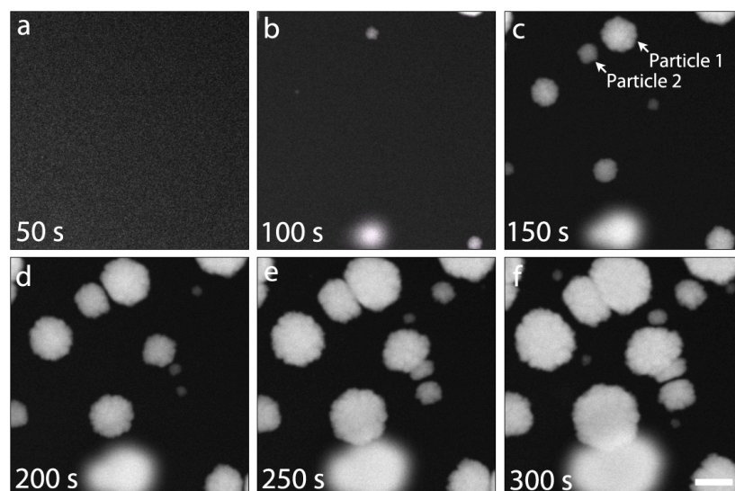
Figure 1. a-f) Time-lapsed ADF STEM images showing the electron beam induced nucleation and growth of Pt from a 1 mM K_2PtCl_6 + 0.5 M H_2SO_4 solution. The electron dose rate is 196 e^-/nm^2s and the scale bar is 200 nm.
