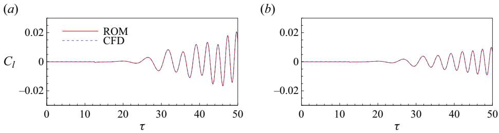
Figure 5. Identified results under the training signal compared with those of direct numerical simulations for (a) Re = 60 and (b) Re = 40 .
