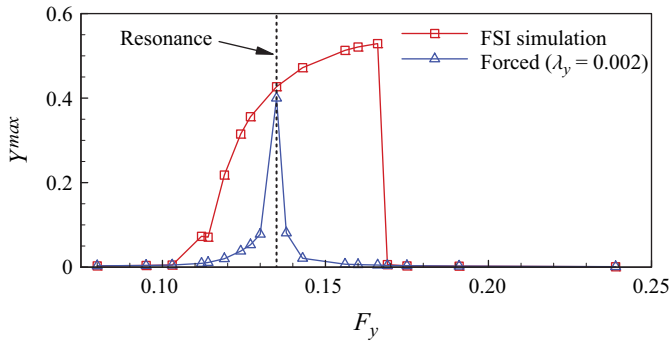
Figure 21. Transverse vibration amplitude of the cylinder as a function of the reduced natural frequency obtained by FSI simulation and forced response simulation.
