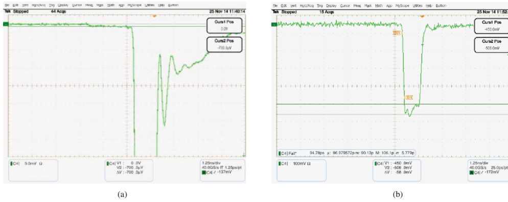
Figure 15. The high contrast temporal waveform (600 : 1). (a) Low amplitude pedestal; (b) high amplitude step.
