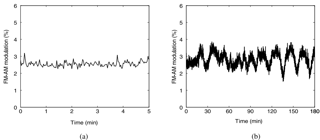
Figure 22. FM-to-AM changes of single polarization front-end system (a) for 5 minutes and (b) for 3 hours.
