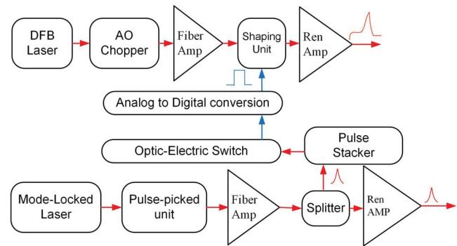
Figure 11. Improved optically driven synchronization schematic.
