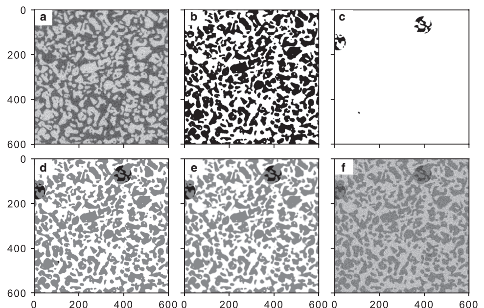
Fig. 4. An overview of the steps used to create the synthetic images: (a) uncast image of S1_I, (b) segmented version of the uncast grayscale image (this is the truth image), (c) air phase generated by the boolean model after correction for the existing ice structure, (d) ideal three-phase image, (e) blurred three-phase image and (f) final synthetic image after addition of scaled \mu\text{CT} noise. The axes' units are voxels.
