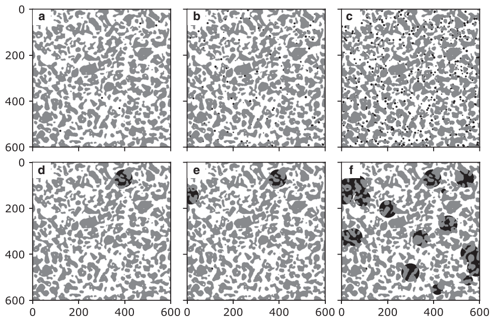
Fig. 6. An overview of the synthetic air bubble configurations generated. All images are based on the S1_I sample and the ideal three-phase image is used for clarity. Structures in (a), (b) and (c) were generated with an air bubble radius of 5 voxels and nominal air volume fractions of 0.001, 0.02 and 0.1, respectively. Structures in (d), (e) and (f) were generated with an air bubble radius of 40 voxels and nominal air volume fractions of 0.001, 0.02 and 0.1, respectively. The axes' units are voxels.
