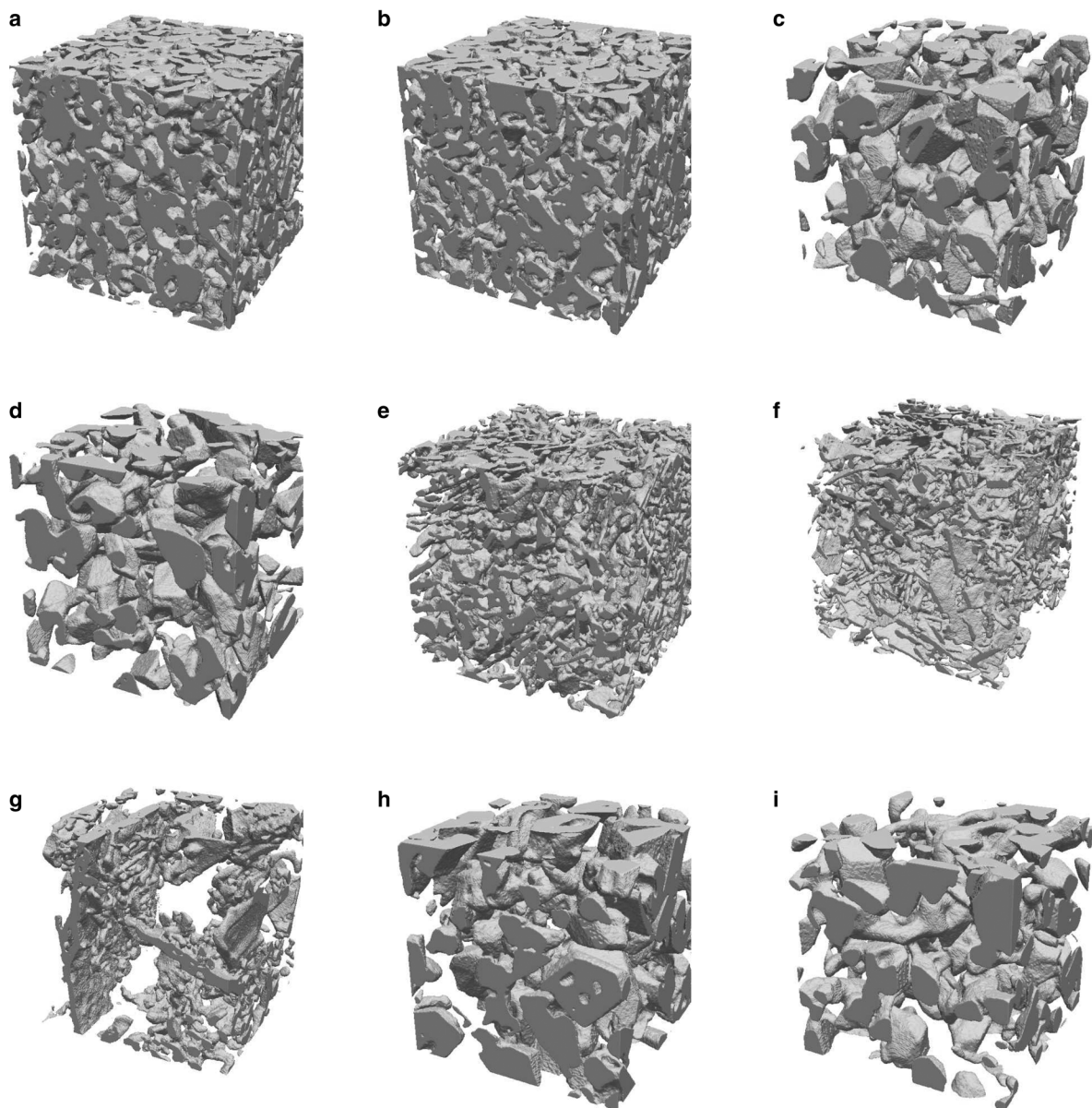
Fig. 1. 3D images of the snow samples used: (a) S1_I, (b) S1_B, (c) S2_I, (d) S2_B, (e) S3_B, (f) S4_B, (g) S5_B, (h) S6_I and (i) S6_B. All volumes are 300 \times 300 \times 300 voxels (300 voxels = 5.4 mm), except for g), which is 500 \times 500 \times 500 voxels (500 voxels = 9.0 mm) in order to capture the large, vertical structures.
