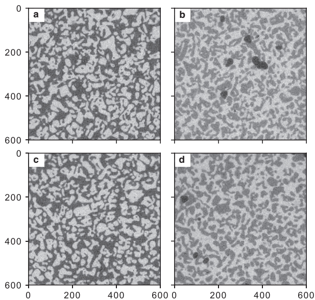
Fig. 2. Representative images of the S1 samples prior to and after casting: (a) S1_B prior to casting, (b) S1_B after casting with BaTiO 3 , (c) S1_I prior to casting and (d) S1_I after casting with I 2 . Note that the respective pre- and post-casting structures are slightly different even though the same region of all samples is shown. This is due to small shifts in the samples between scans. The axes' units are voxels.
