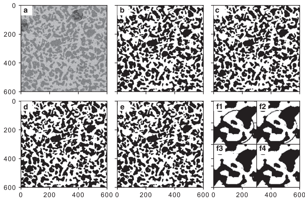
Fig. 7. An example of the segmentation steps for a synthetic image of S1_I with an air bubble radius of 40 voxels and a nominal air volume fraction of 0.02. The steps are shown as (a) starting grayscale synthetic image, (b) segmented image after the Gaussian filter, (c) segmented image after distance mapping, (d) segmented image after gradient thresholding, (e) final segmented image (i.e. after component labeling) and (f1–f4) zoomed in views of an air bubble from (b), (c), (d) and (e), respectively. The axes' units are voxels.
