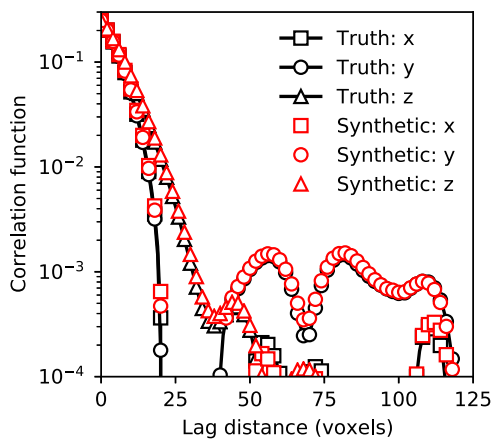
Fig. 9. The correlation function for synthetic and truth images of the S1_I sample with air bubble volume fraction of 0.02 and radius of 40 voxels.
