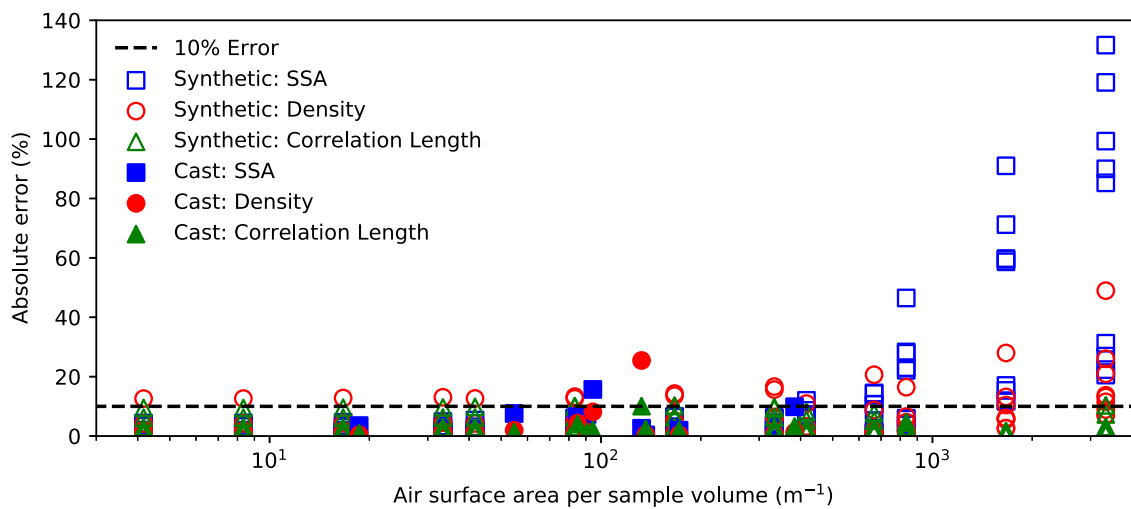
Fig. 11. A summary of the absolute error of SSA, density and correlation length for all synthetic and cast images as a function of ASAV. The ASAV is the nominal value for the synthetic images and calculated for the cast images. The error is with respect to the truth and uncast values for the synthetic and cast images, respectively.
