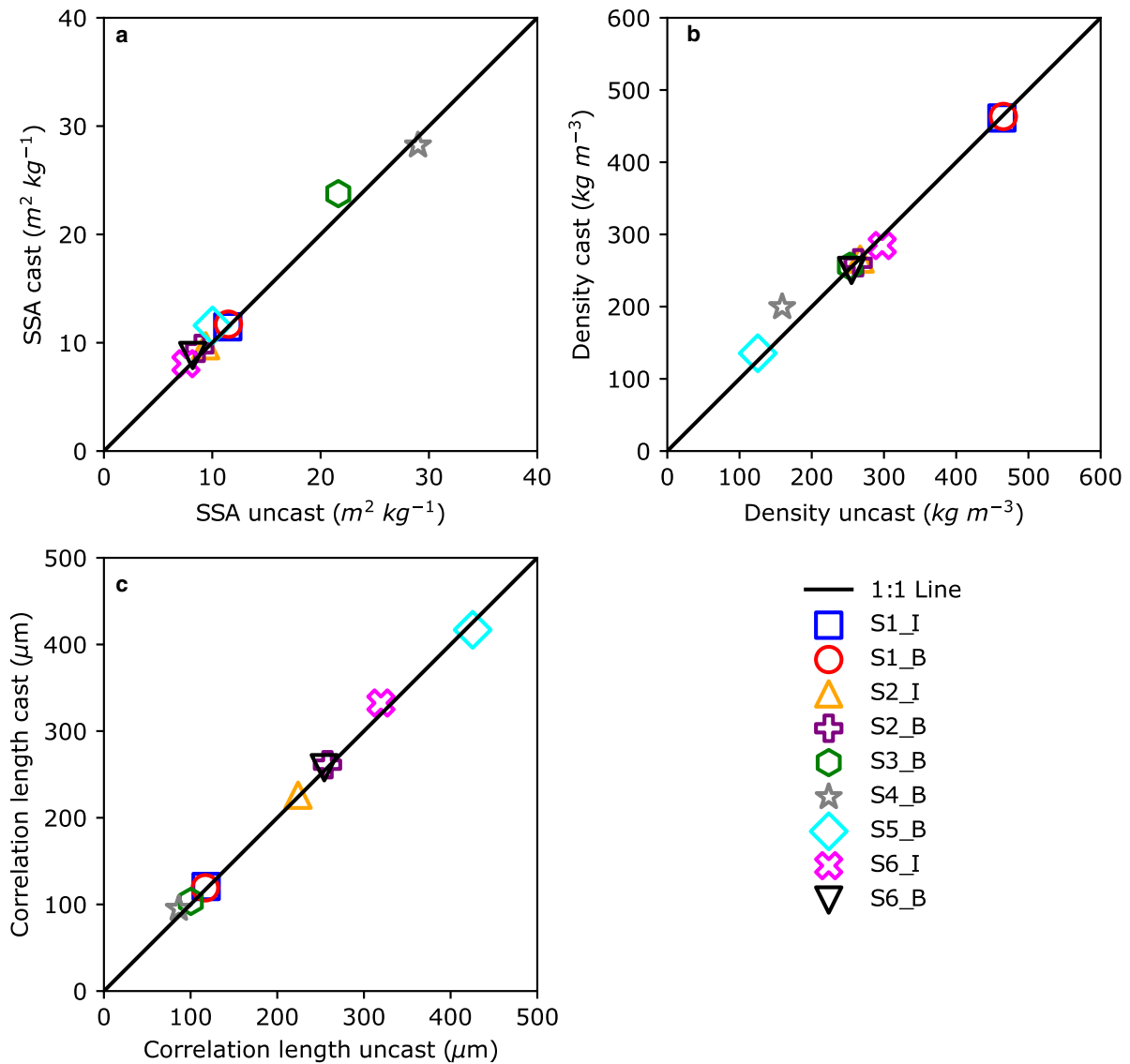
Fig. 10. Results of the comparison between the uncast and cast images for (a) SSA, (b) density and (c) correlation length.
