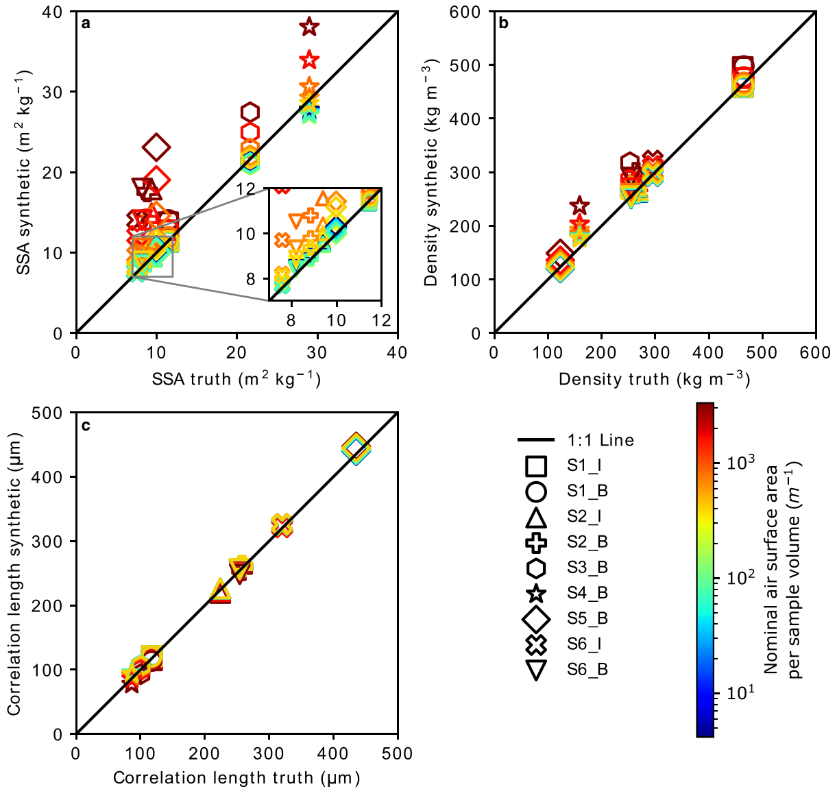
Fig. 8. Results of the synthetic comparison between the truth and synthetic images for (a) SSA, (b) density and (c) correlation length. The color bar in the lower right applies to all three plots.
