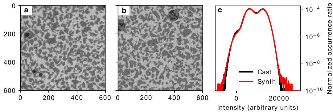
Fig. 5. A comparison of (a) the cast image of S1_I, (b) the synthetic image of S1_I with a nominal air volume fraction of 0.02 and radius of 40 voxels and (c) the resulting histograms. The axes' units in (a) and (b) are voxels.
