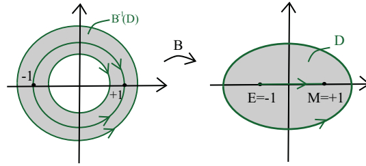
FIGURE 1. Birkhoff regularization.
