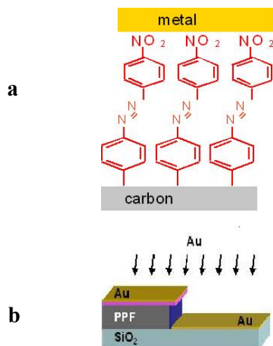
Figure 1. Schematic Diagrams of a: Au-NAB-Si multilayer device b: side wall Au-NAB-PPF junction
