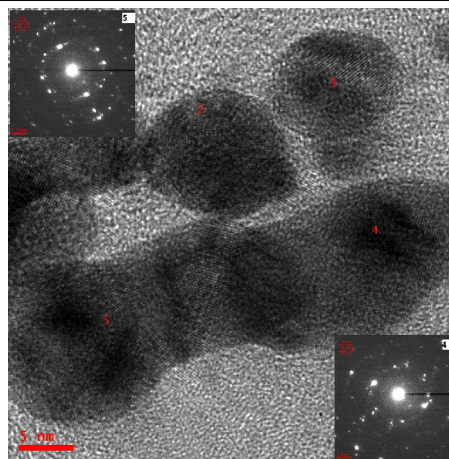
Figure 4. HR TEM images of Au particles on side wall junctions. Inserts are NBD patterns from individual particles (No.4 and No.5 in the image).
