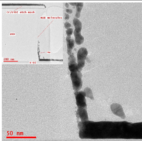
Figure 3. BF TEM images of side wall junctions, showing non-continuous Au films on side walls – insert is a low mag. Image of the whole side wall cross section.
