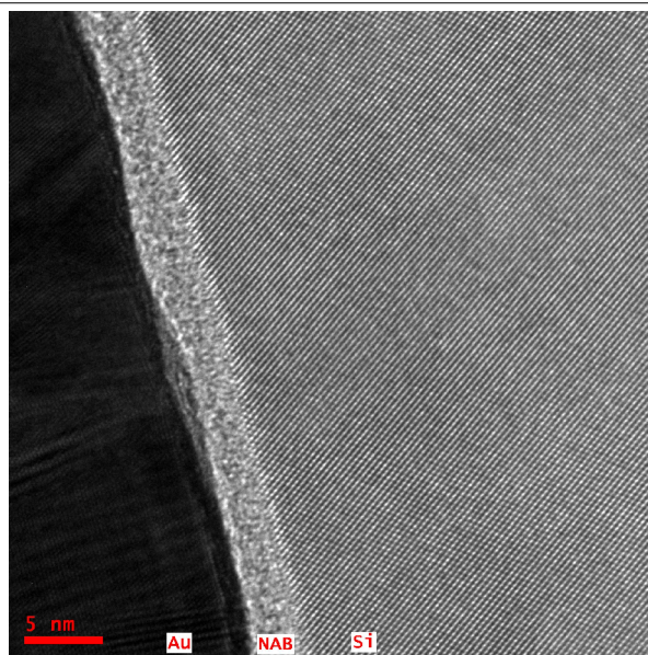
Figure 2. HRTEM images of Au/NAB/Si interfaces.
