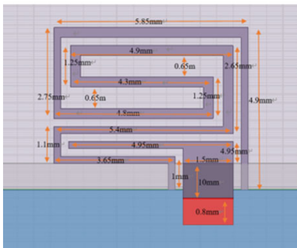
Figure 1. (a) The position of the MIMO antenna array in a mobile phone; the detail parameters for the proposed single antenna element in (b) the front view and (c) the lateral view.
