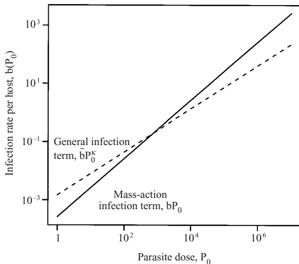
Fig. 3. Comparing the infection terms of the fitted mass-action infection model (equation 10), bP_0 , (solid line) and the fitted general infection model (equation 12), \tilde{b}P_0^\kappa (dashed line). For low parasite doses, the general infection model (equation 12) predicts higher rates of infection, and for high parasite doses lower rates of infection than the mass-action infection model (equation 10). The infection terms coincide at approximately the ID_{50} .
