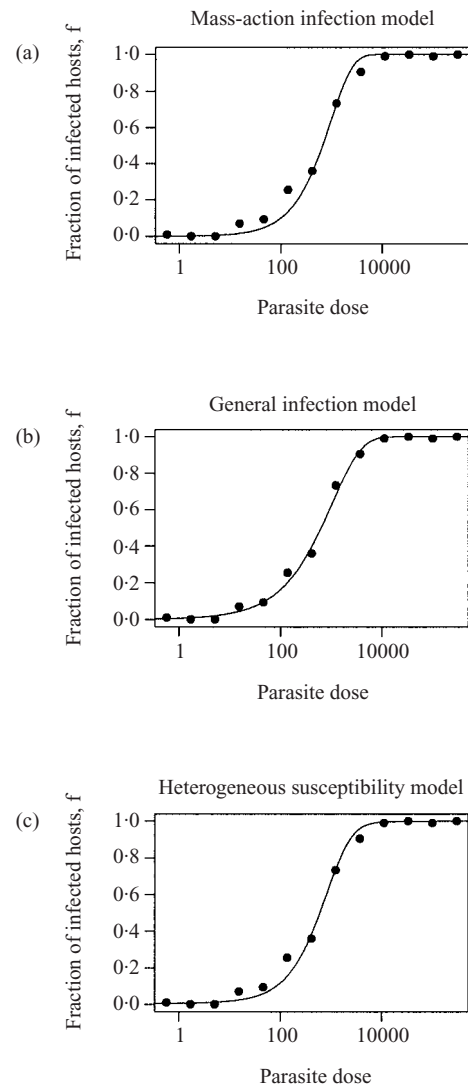
Fig. 2. Fitting (a) the mass-action infection model (equation 10), (b) the general infection model (equation 12), and (c) the heterogeneous susceptibility model (equation 13) to our dataset. The mass-action infection model (equation 10) is largely consistent with the data, but overestimates the slope of f at intermediate parasite doses. The general infection model (equation 12) and the heterogeneous susceptibility model (equation 13) fit significantly better ( F -test on the residual sum of squares: p = 0.00036 and p = 0.021 , respectively).
