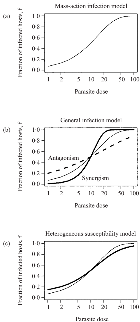
Fig. 1. Theoretical expectations for the fraction of infected hosts, f , as a function of the parasite inoculum, P_0 : (a) the mass-action infection model (equation 10), (b) the general infection model (equation 12) that incorporates synergistic/antagonistic interaction between the parasites during the infection process, and (c) the heterogeneous susceptibility model (equation 13) that assumes normally distributed host susceptibilities. The thin line in (b) and (c) shows the mass-action infection model (equation 10) for comparison.
