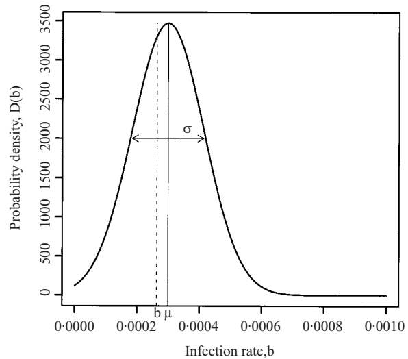
Fig. 4. Estimated distribution of host susceptibilities. The estimate of the infection rate b of the mass-action infection model (equation 10) is also plotted for comparison.
