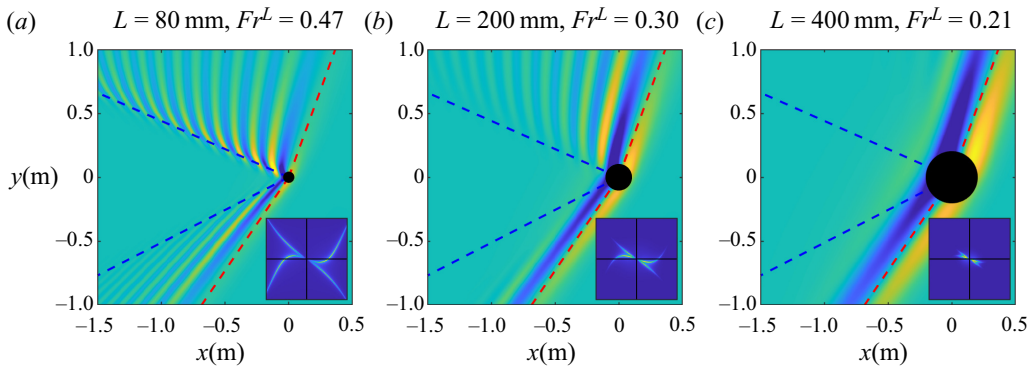
Figure 7. Theoretical wakes (and their associated Fourier transform) on the layered bathymetry with the parameters h_x = 12 mm, h_y = 47.5 mm, \alpha = -39^\circ and a ship speed U = 0.42 ms -1 . The size of the ship L varies from 80 to 400 mm (2 to 10 times the ship size in the experiments), with associated hull Froude number Fr^L from 0.47 to 0.21. The dashed curves indicate the schematic representation of the wake.
