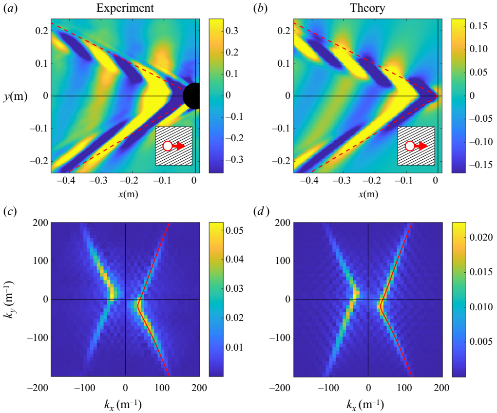
Figure 6. Surface elevation for the parameters h^- = 10 mm, h^+ = 55 mm, h_x = 12 mm, h_y = 47.5 mm, \alpha = -62^\circ and U = 0.47 ms -1 . (a) Experimental results (wave amplitude in mm); the red dashed lines indicate the maximum angle of the wake; the inset shows the layered bathymetry with the red arrow indicating the ship propagation. The colour scale is saturated to emphasize the transverse waves. (c) Fast Fourier transform of the experimental results; the red curve corresponds to the theoretical dispersion relation (2.2) and (2.3). (d) Theoretical wave amplitude obtained by Fourier transform (discretization of (A2)) and (b) the coefficients of its discrete inverse both with arbitrary amplitude.
