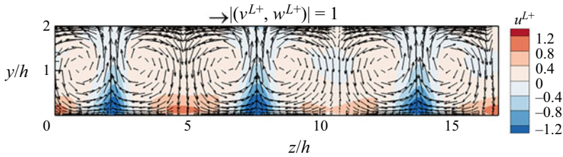
Figure 24. Instantaneous field of u_i^L in case 8 with La_t = 0.3 . The contours are u^{L+} and the vectors are (v^{L+}, w^{L+}) .
