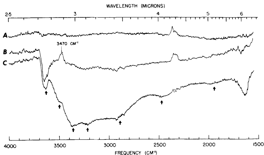
Fig. 1. Differential i.r. spectra of lithium nitrate treated muscovite after hydrogen saturation. A—Matched specimens in air-dry state; B—specimen in reference beam heated to 300°C, specimen in sample beam heated to 160°C; C—specimen in reference beam heated to 300°C, specimen in sample beam in air-dry state. Arrows indicate significant OH stretching bands for adsorbed water on air-dry mica.
