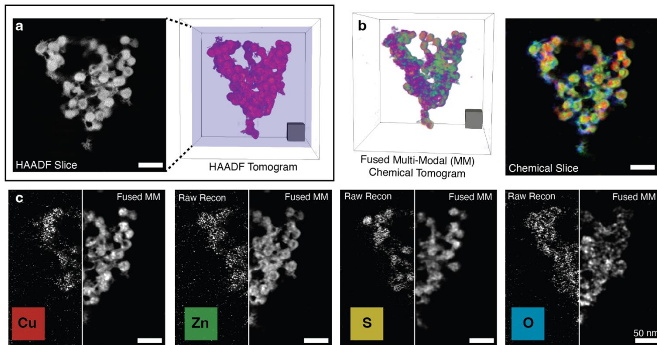
Figure 2: Demonstrating fused multi-modal electron tomography on ZnS/CuS nanoparticles. a, The HAADF reconstruction with a 2D slice shown on the left. b, The fused multi-modal reconstruction illustrating CuS or ZnS rich nanoparticles and oxidized shells. c, 2D slices of the chemical reconstructions with the noisy traditional reconstructions highlighted on the left of each image.
