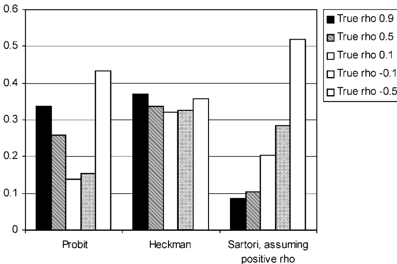
Fig. 4 RMSEs of estimates of \beta_2 .
