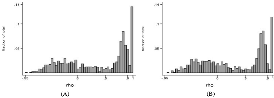
Fig. 3 Histogram of Heckman’s estimates of \rho : true \rho is (A) .9 and (B) .5.
