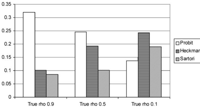
Fig. 6 RMSEs of \hat{\beta}_2 when a stronger (but still weak) exclusion restriction is valid.
