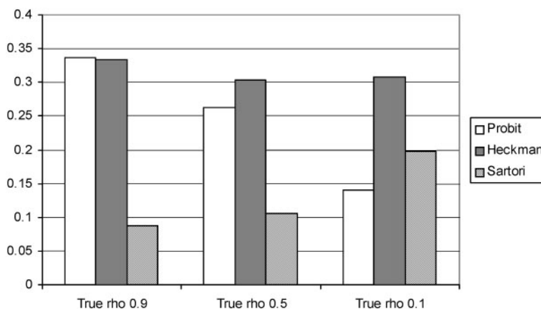
Fig. 5 RMSEs of \hat{\beta}_2 when a very weak exclusion restriction is valid.
