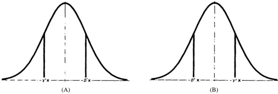
Fig. 1 The distribution of u_i when (A) -\gamma'x_i < -\beta'x_i and (B) -\beta'x_i < -\gamma'x_i .
