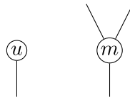
FIGURE 1. Generating operations of \text{Ass}^{\text{un}} .
