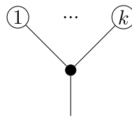
FIGURE 5. Image of \underline{x_1 \cdots x_k} .
