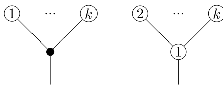
FIGURE 4. Generating operations of \text{Br}_{\mathcal{C}} .
