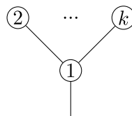
FIGURE 7. Image of x_1 \wedge \underline{x_2 \cdots x_k} .
