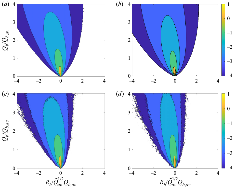
Figure 10. Logarithms of joint p.d.f.s of Q_b/Q_{b,av} and R_b/\tilde{Q}_{av}^{1/2} Q_{b,av} from (a) DNS1, (b) DNS2, (c) M1, and (d) M2. Colours indicate the values of the decimal logarithm of the p.d.f.
