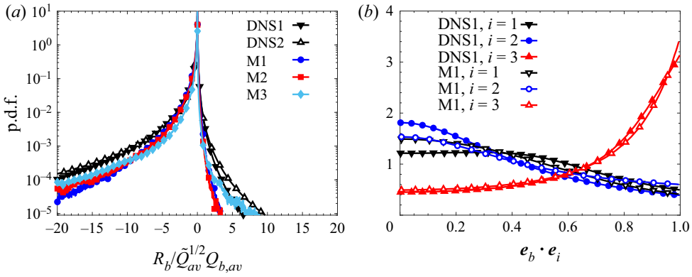
Figure 7. The p.d.f.s of (a) R_b / \tilde{Q}_{av}^{1/2} Q_{b,av} and (b) the inner product between the unit vector e_b \equiv \mathbf{b} / \|\mathbf{b}\| and the eigenvectors e_i of \mathcal{S} .
