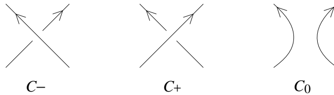
Fig. 1.13 The possible (non)crossings.
