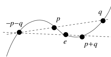
Fig. 2.6 Addition of points on a cubic.
