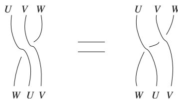
Fig. 1.27 The hexagon axiom revisited.
