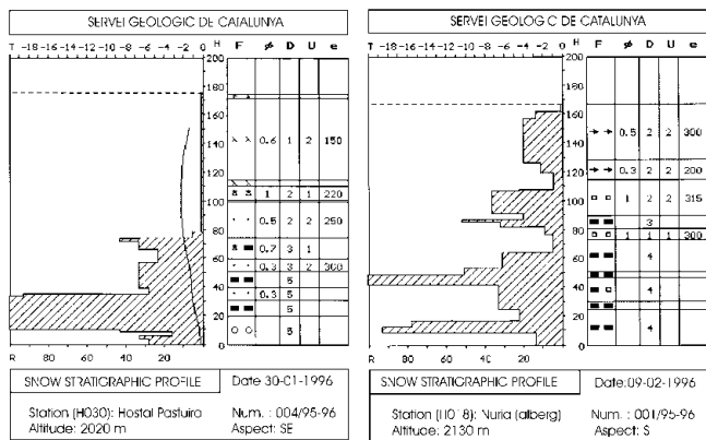
Fig. 3. Snow stratigraphic profiles; T: Temperature (°C); H: snow height; F: snow-grains form; φ: snow-grains diameter; D: snow hardness (qualitative); U: snow humidity (qualitative); e: snow density. Symbols correspond to the international classification for seasonal snow on the ground (Colbeck and others, 1990). (a) Snow profile corresponding to the second snowstorm period before the 7–8 February 1996 avalanche. It was recorded at Hostal Pastuira (2020 m a.s.l.), located about 10 km east of Vall de Núria but in the same climatic region. The new snow accumulated during this period was about 100 cm in this location. (b) Snow profile corresponding to the third snowstorm period before the 7–8 February 1996 avalanche. It was recorded at Vall de Núria (2130 m a.s.l.). The new snow accumulated during this period was about 60 cm in this location.
