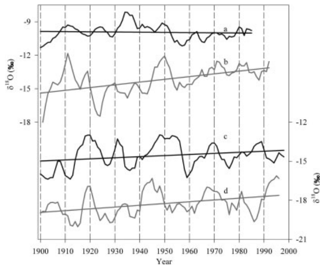
Fig. 4. The 3 year running averaged \delta^{18}\text{O} records for the four ice cores from the TP presented in the paper: (a) Dundu, (b) Guliya, (c) Puruogangri and (d) Dasuopu. The trend lines of Guliya, Puruogangri and Dasuopu show obvious warming since 1900, but the Dundu warming is less obvious because the record ends in 1985.
