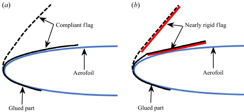
Figure 3. Schematic of the aerofoil–flag assembly for (a) compliant flags, and (b) nearly rigid flags.
