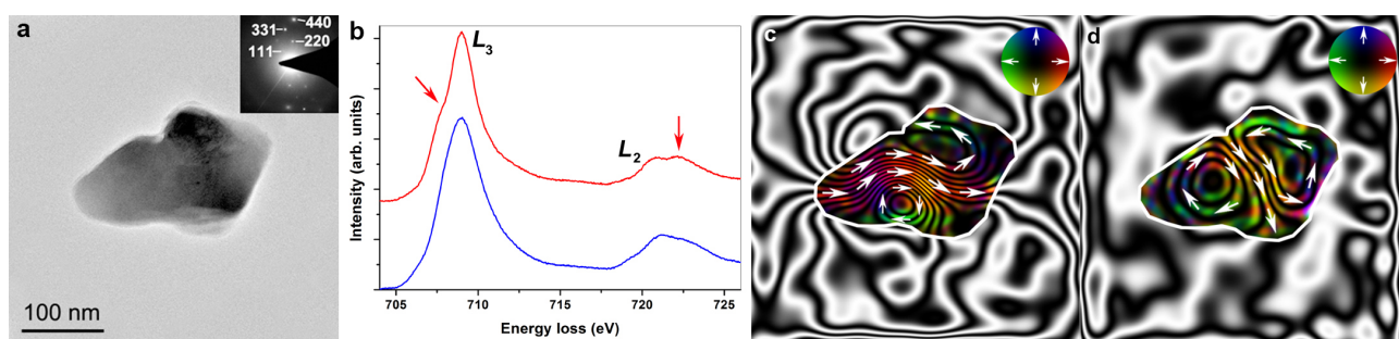
Figure 1. (a) TEM image of an \text{Fe}_3\text{O}_4 particle and (b) EEL spectra acquired before (blue) and after (red) oxidation. (c, d) Magnetic induction maps of the particle (c) before and (d) after oxidation [1].
