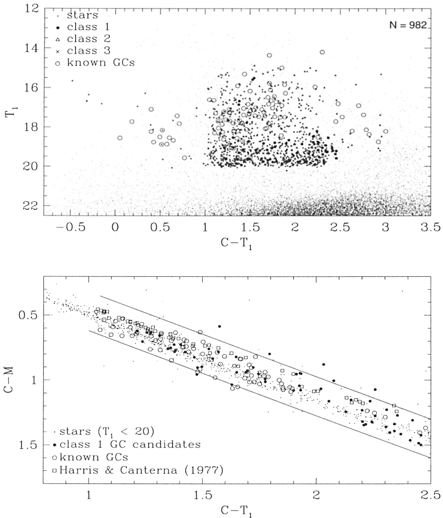
Figure 2. Color-magnitude diagram (upper panel) and color-color diagram (lower panel) of new GC candidates. Stars of one field are plotted as small dots. Class 1 (probable GCs), class 2 (possible GCs) and class 3 (doubtful GCs) objects are plotted by filled circles, triangles, and \times 's, respectively. Open circles present \sim 100 known GCs in M31. Open squares in the color-color diagram are GCs in the Galaxy, Fornax dSph, and M31 taken from Harris & Canterna (1977). Objects deviating much from the main locus need further checking.
