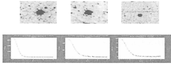
Figure 1. (Upper panel, from left to right) T_1 images ( 34'' \times 34'' ) of a star ( T_1 = 14.3 , C - T_1 = 1.2 ), a known GC (315-038, V = 16.3 , B - V = 0.4 ), and a new GC candidate ( T_1 = 19.3 , C - T_1 = 1.4 ). (Lower panel, from left to right) Radial profiles of the star, the known GC, and the new GC candidate. Note that the FWHM of the star and the typical FWHM of the image is 1.8 px. The FWHM of the known GC is 2.6 px, and that of the new GC candidate is 2.8 px.
