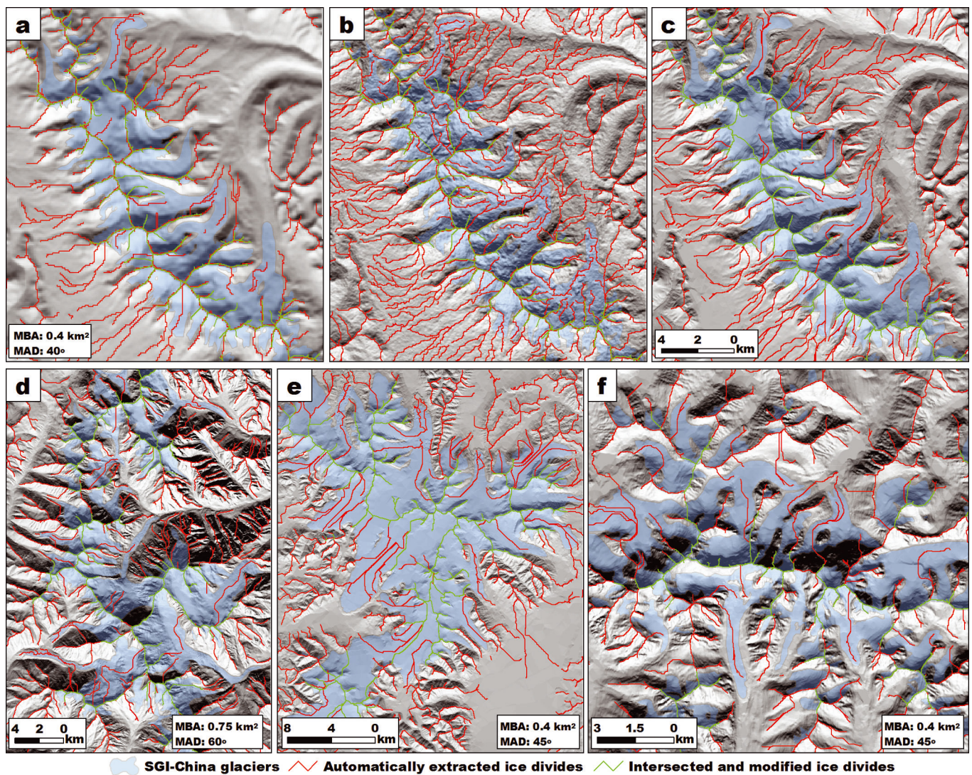
Fig. 4. Ice divides in Anyemaqen mountains, Qinghai Province, extracted from (a) SRTM, (b) GDEM2 and (c) 1 : 50 000 topo-DEM. The intersected and modified ice divides in (c) are shown in (a) and (b) for comparison. The other examples are ice divides extracted from 1 : 50 000 topo-DEMs for (d) Gongga mountains, Sichuan Province, (e) Purogangri, Tibet Province, and (f) Bogda mountains, Xinjiang Province. MBA and MAD are the minimum basin area and minimum aspect difference, respectively.
