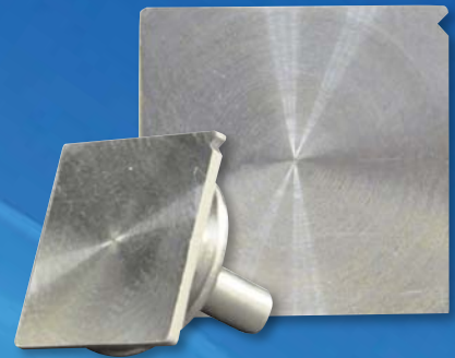
PELCO® Q Pin Stubs for Correlative Microscopy
