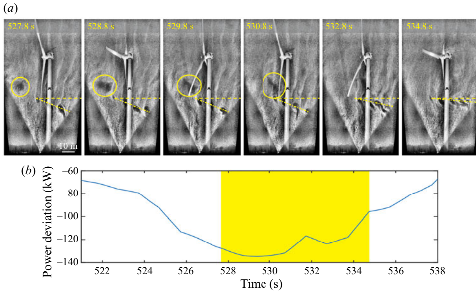
Figure 10. Example of a coherent structure interacting with the turbine and inducing (a) a reduction in wake expansion and (b) a reduction in power generation. In (a), the coherent structure is circled in yellow, and the wake expansion angle is indicated by the yellow lines. The dashed line represents the bottom blade tip elevation, and the dot-dashed line shows the position of the tip vortices. The yellow region marked in (b) indicates the time period shown in the images. Power deviation is defined as the expected power production at the given wind speed based on the power curve, subtracted from the actual power produced.
