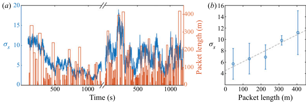
Figure 9. Relationship between coherent structure packet length and standard deviation of lateral tower strain ( \sigma_s ), including (a) a time series across both Feb 2019 datasets, and (b) a scatter plot with the \sigma_s data points binned by packet length. The circles indicate the mean value of \sigma_s for each value of packet length, and the error bars indicate the standard deviation. Once again, the Apr 2018 dataset has been removed due to the limited duration of turbine operation (3 %).
