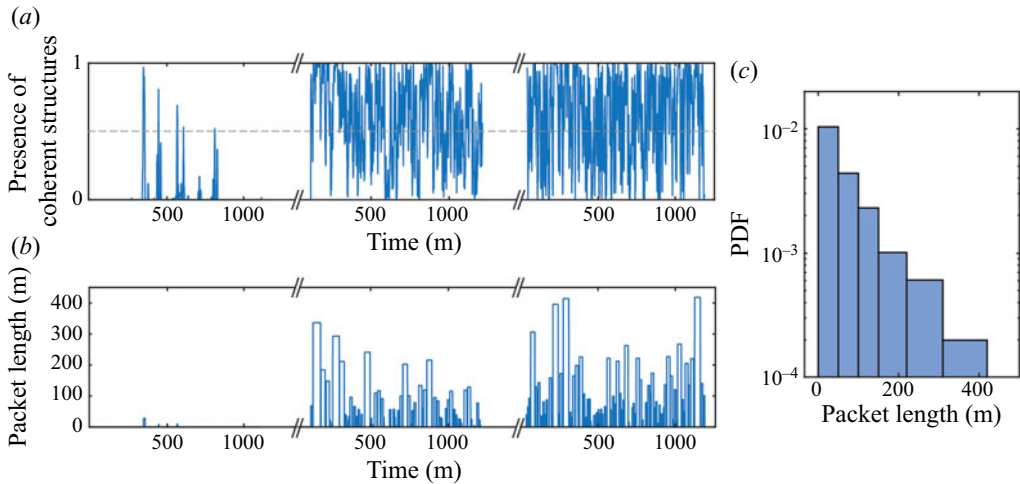
Figure 5. (a) The level of coherent structures from image classification, with a dashed grey line indicating the threshold, used to determine (b) the coherent structure packet length scale. (c) The PDF of the packet length for all three datasets. Note that the bin size is gradually increased for events with larger packet lengths to ensure sufficient statistical convergence for events with lower probability of occurrence.
