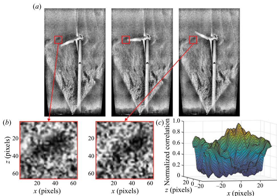
Figure 3. Demonstration of the PIV blade-skipping algorithm, including (a) sample images with one PIV window ( 64 \times 64 pixels) outlined in red. The first image is the frame before the blade enters the window, the second is a frame with the blade inside the window and the third is the frame just after the blade moves outside the window. The windows from the first and third images, exhibiting a clear pattern persisting across the frames, are shown in (b), and their correlation is shown in (c).
