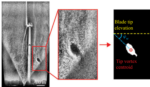
Figure 11. Definition of wake expansion angle, \varphi_w , as determined using the centroid of the bottom blade tip vortex and the elevation of the tip of the bottom turbine blade.
