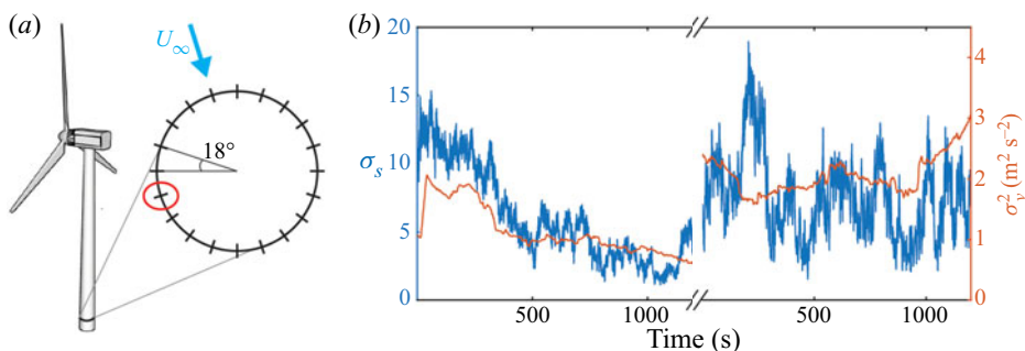
Figure 7. (a) Schematic showing the strain gauges located around the base of the Eolos turbine tower. The strain gauge used for the following analysis is circled in red and the wind direction is indicated by a blue arrow. (b) Time series of the standard deviation of strain ( \sigma_s ) and the square of the standard deviation of the spanwise wind component ( \sigma_v^2 ) for both Feb 2019 datasets. Note that the Apr 2018 dataset has been removed, as the turbine is not producing power for 97% of the recorded period.
