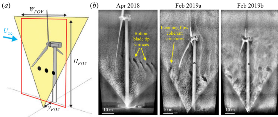
Figure 1. (a) Schematic showing the flow visualization FOV for the experiments. (b) Sample enhanced and de-warped flow visualization images for each of the three datasets. Arrows indicate vortices shed from the bottom blade tips in the near wake and coherent structures in the inflow, both seen as voids in the snow images.
