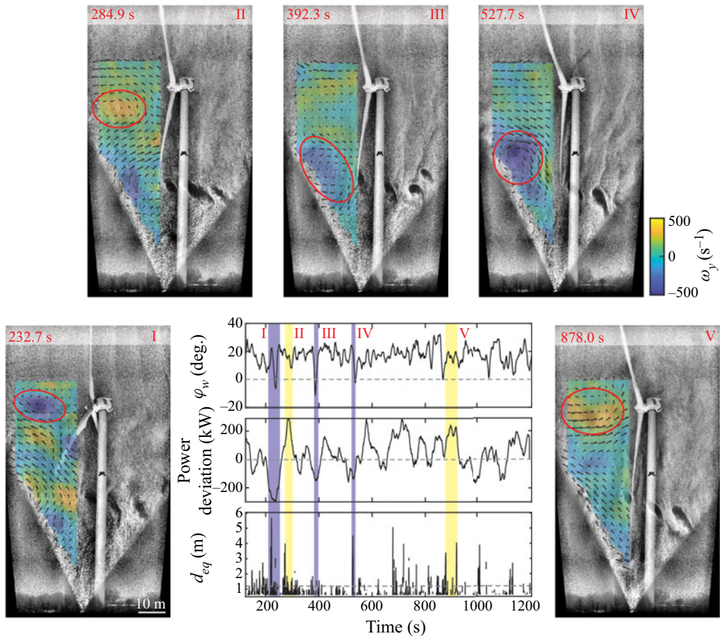
Figure 12. Time series of wake expansion angle ( \varphi_w ), power deviation (expected power subtracted from actual power) and vortex size ( d_{eq} ). The blue and yellow bars indicate periods with strong power deficits and surpluses, respectively. The red numbers correspond to the images show around the plot, which are sample enhanced snow particle images superimposed with spanwise vorticity and vector fields from each highlighted time period. The vector fields represent the fluid velocity with the mean subtracted. Note that the region of positive vorticity around the bottom blade tip in some images is caused by recently generated tip vortices. Supplementary movies 1–5 are available at https://doi.org/10.1017/flo.2021.20 show the vorticity and vector fields for the duration of each of the five highlighted periods.
