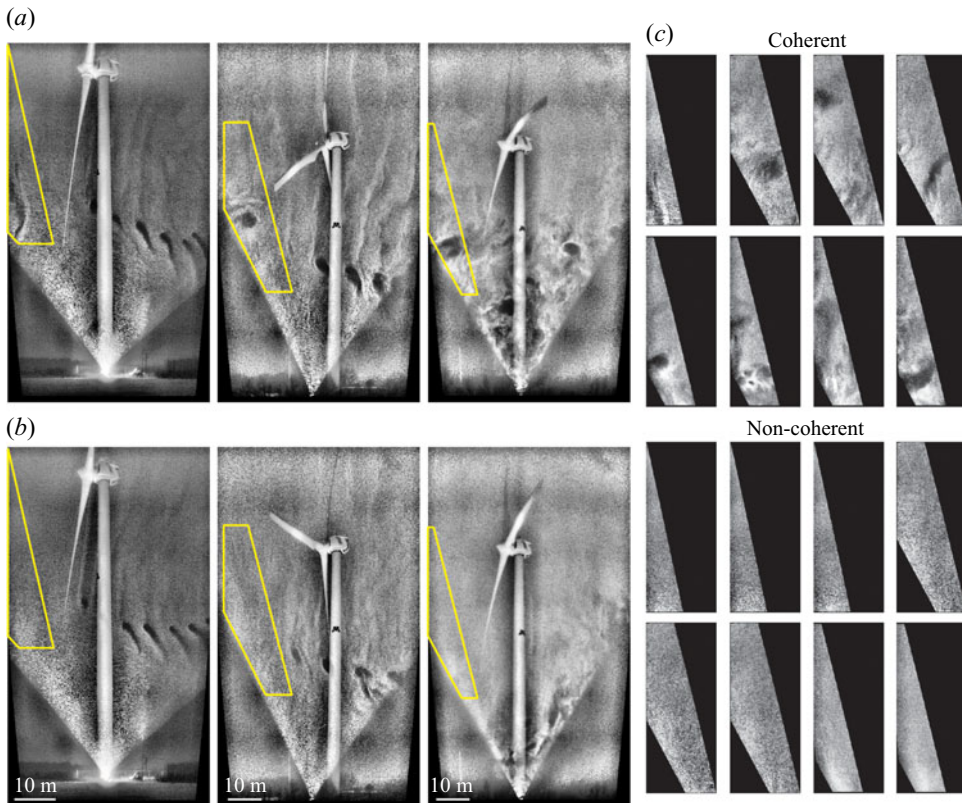
Figure 2. Sample frames for each of the three datasets (a) with coherent structures and (b) without coherent structures in the inflow. The yellow outline indicates the region used for the machine learning classification. Note that the physical locations of these sampling regions are the same for all three datasets, although they appear different due to the differences in the FOVs. (c) A gallery of example coherent and non-coherent images used to train the classifier.
