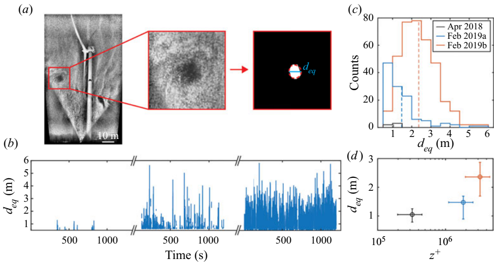
Figure 6. Vortex size characterization, including (a) a sample image with a coherent structure in the inflow, and the resulting extracted void. The equivalent diameter ( d_{eq} ) of the void is indicated by the blue line bisecting the red dashed circle. (b) A time series of d_{eq} over all three datasets. (c) Histogram of d_{eq} for each dataset, with dashed vertical lines representing the mean. (d) Relationship between z^+ and d_{eq} , with the circles indicating the mean values and the error bars representing the standard deviations. A log scale is used for z^+ , as ABL quantities typically vary with the log of the elevation.
