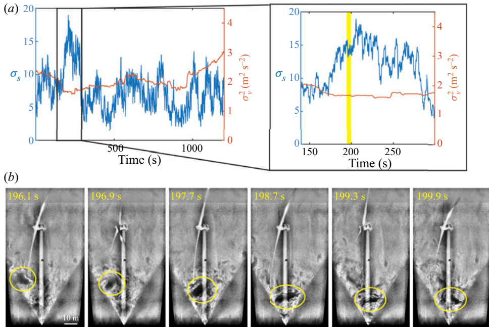
Figure 8. Effect of coherent structures on tower strain, including (a) an example of \sigma_s deviating from \sigma_v^2 . The yellow bar indicates the time range of the images shown in (b), which highlight an atmospheric coherent structure (circled in yellow) impinging on the turbine tower. Several such structures were observed during this period of increased \sigma_s , although only the clearest is shown here.
