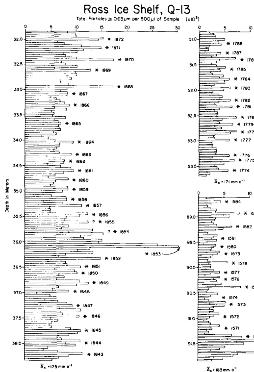
Fig.2. Total particle concentration in three sections of the Q-13 core. Dates were assigned by counting the cyclical variations in microparticle concentration. \bar{A}_n is the average annual accumulation rate for each section.
