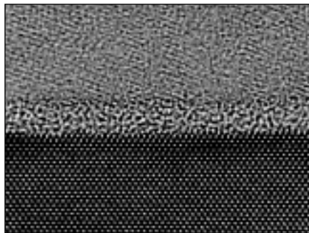
High-resolution transmission electron microscopy image showing a 1.6-nm gate oxide. (Credit: Frieder Baumann, Lucent Technologies/Bell Labs.)
