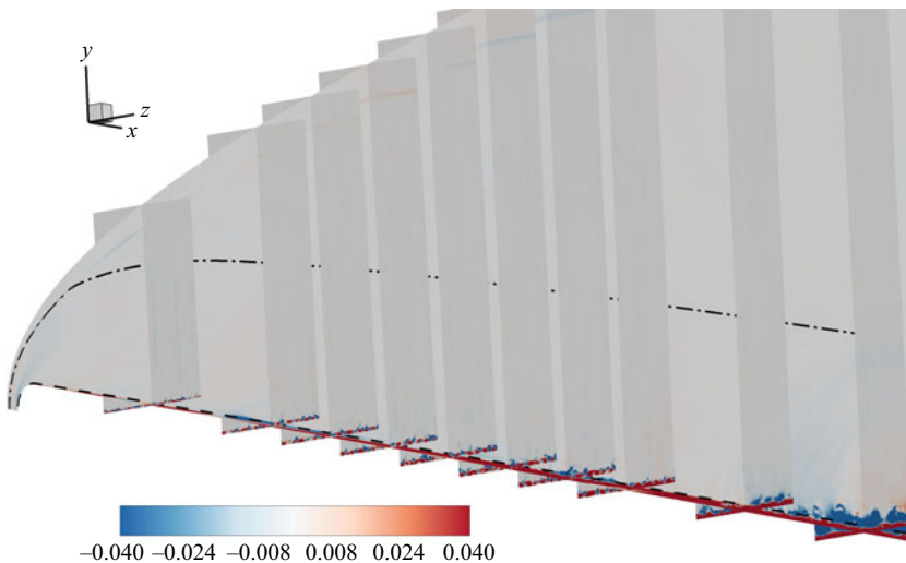
Figure 31. Contour of the streamwise velocity perturbation u_{perturb} compared to the laminar flow for case R3 at t = 806 . Dashed and dash-dotted lines mark the boundary-layer edge and the entropy-layer edge, respectively. Transverse slices are extracted and shown with x -coordinates 20, 40, 50, 60, 70, 80, 90, 120 and 140, successively.
