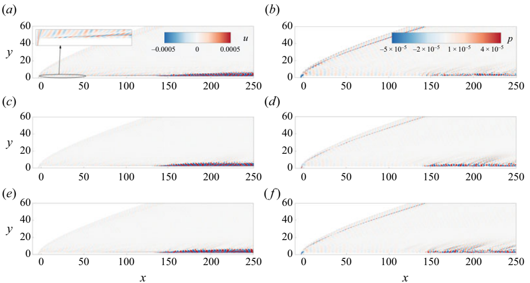
Figure 23. (a,c,e) Streamwise velocity and (b,d,f) pressure for the first, second and third leading SPOD x - y modes from top to bottom at f^* = 120 kHz for case R2C.
