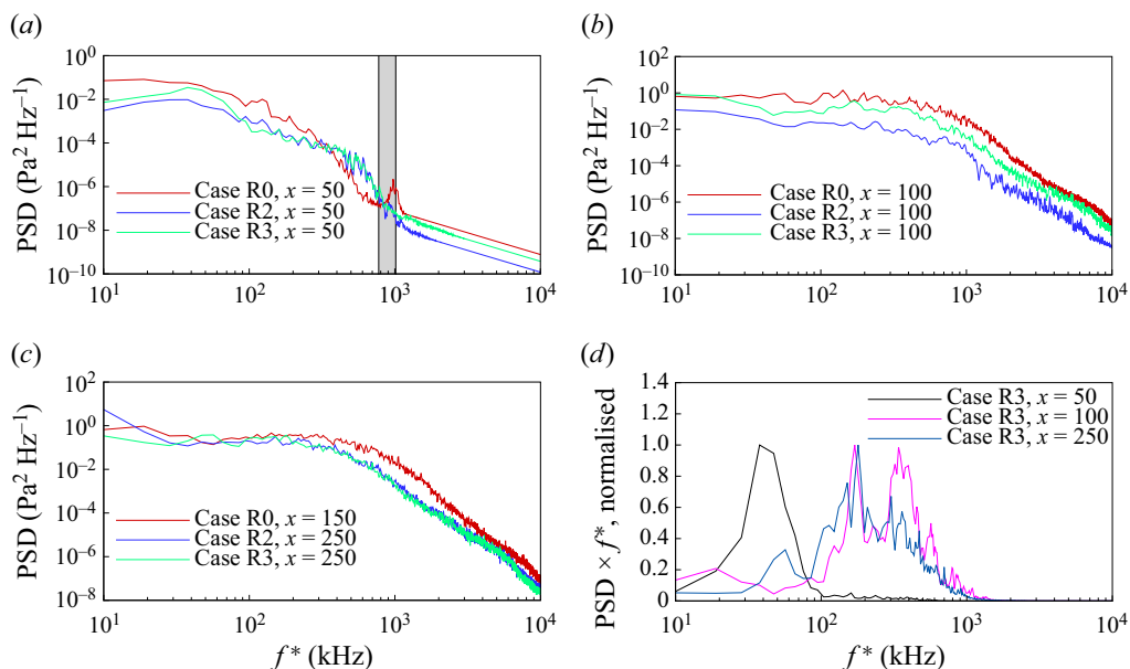
Figure 21. Temporal PSD of the wall pressure fluctuation probed along z = L_z/2 in (a) pre-transitional, (b) transitional and (c) nearly turbulent regions. (d) Premultiplied PSD normalised by each maximum for case R3. The grey area in (a) represents the frequency range of the unstable second mode given by LST.
