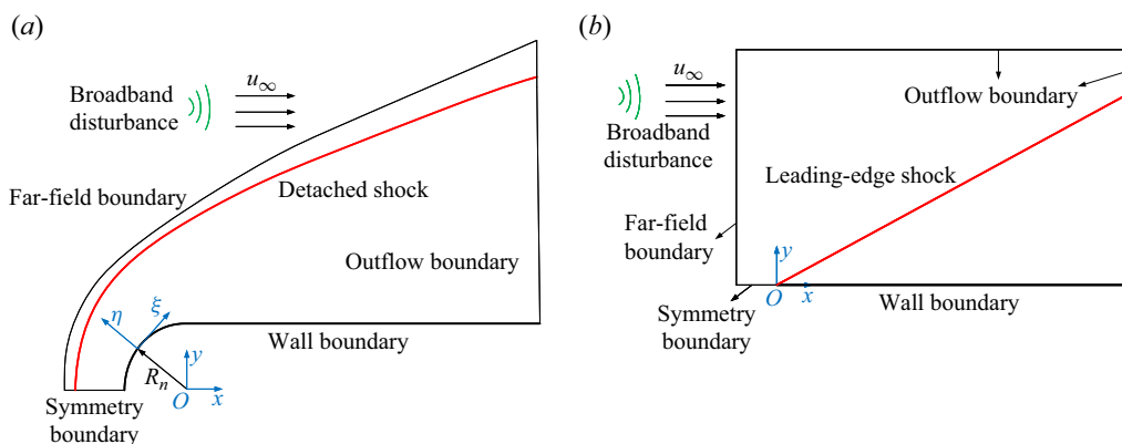
Figure 1. Schematic drawings of the simulated flow over (a) a blunt plate and (b) a sharp-leading-edge plate (not to scale).
