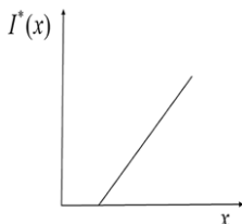
Figure 3. Y \uparrow_{SPED} X and Z is independent of X .
