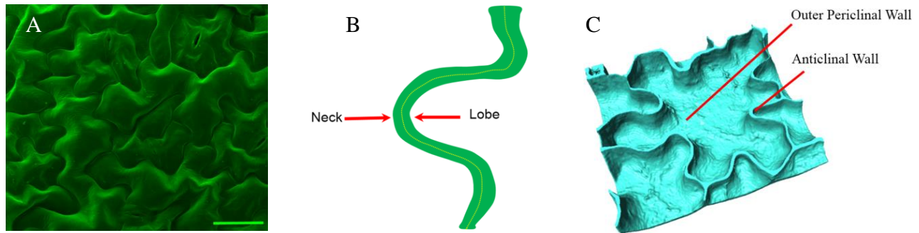
Figure 1. a) Scanning electron micrograph of Arabidopsis leaf pavement cells. Scale bar = 30 \mu\text{m} b) Definition of a pair of lobe and neck in a wall undulation c) Rotated 3D reconstruction of 3D stack of confocal micrographs of a pavement cell.
