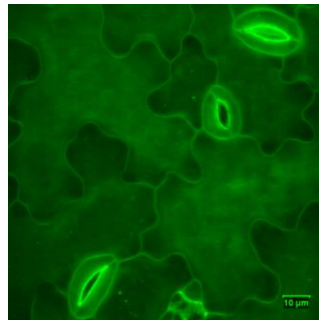
Figure 3. Propidium iodide staining shows presence of de-esterified pectin on the neck side of undulations. Scale bar = 10 \mu\text{m} .
