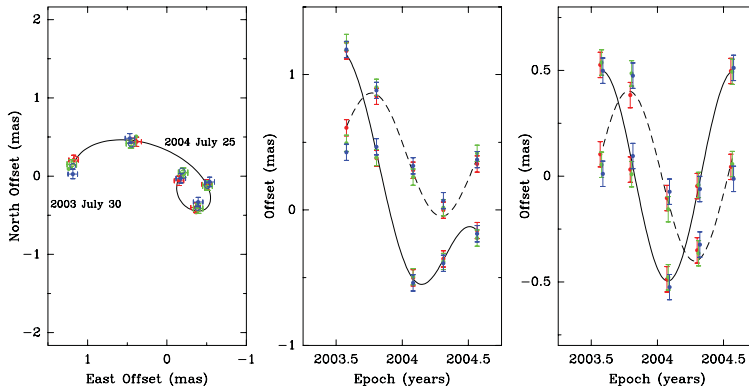
Figure 2. Parallax data for 12 GHz \text{CH}_3\text{OH} masers in W3OH from Xu et al. (2006). Left panel: positions on the sky of 1 maser spot measured relative to 3 background sources. Middle panel: eastward (solid line) and northward (dashed line) offsets versus time. Right panel: same as middle panel, but with proper motion removed, showing only the parallax signature.
