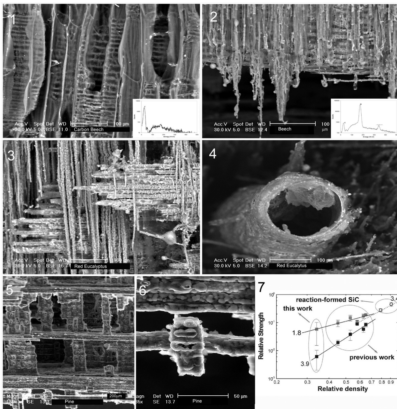
Fig. 1. SEM image and EDS of pyrolyzed/carbonized beech wood showing the fibrous structure. Fig. 2. SEM image and EDS of beech wood after Si infiltration of Si and forming SiC. Fig. 3. SEM images of red eucalyptus wood cut parallel to the former wood precursor. Fig. 4. SEM images of red eucalyptus wood cut perpendicular to the former wood precursor. Fig. 5. SEM images of pine wood revealing the details of interconnected structure. Fig. 6. SEM images close-up view of pine wood showing the detail of the fibrous microstructure. Fig. 7. Comparison of relative strength vs. the relative density of SiC from different sources.
