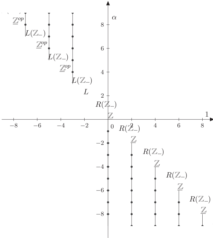
Figure 1. The Mackey functor H\mathbb{Z}_* . Vertical lines represent the product by the Euler class \alpha , and dots represent copies of the Mackey functor \langle \mathbb{F} \rangle .
