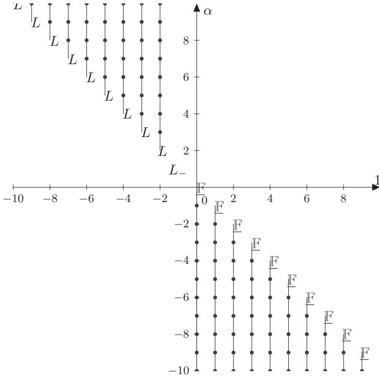
Figure 2. The Mackey functor HF_{\alpha} . Vertical lines represent the product by the Euler class a , and dots represent copies of the Mackey functor (F) .
