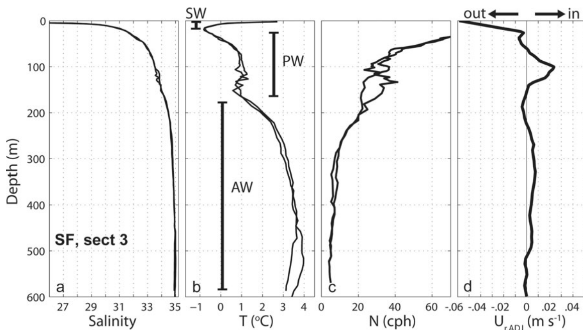
Fig. 2. (a) Two typical salinity versus depth profiles from Sermilik Fjord taken during summer 2009 at section 3 near mid-fjord. (b) As in (a) but for temperature showing approximate depth boundaries of the three main water masses: polar water (PW), Atlantic water (AW) and surface water (SW). (c) As in (a) but showing the buoyancy frequency N in cycles per hour. Note that N has been smoothed with a 10 m running average filter. (d) U_{r,ADJ} profile transformed into depth space for Sermilik Fjord section 3, with arrows indicating in- or out-fjord flow.
